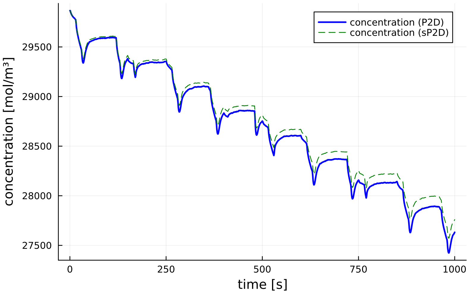
concentration_comparison (P2D vs sP2D)
