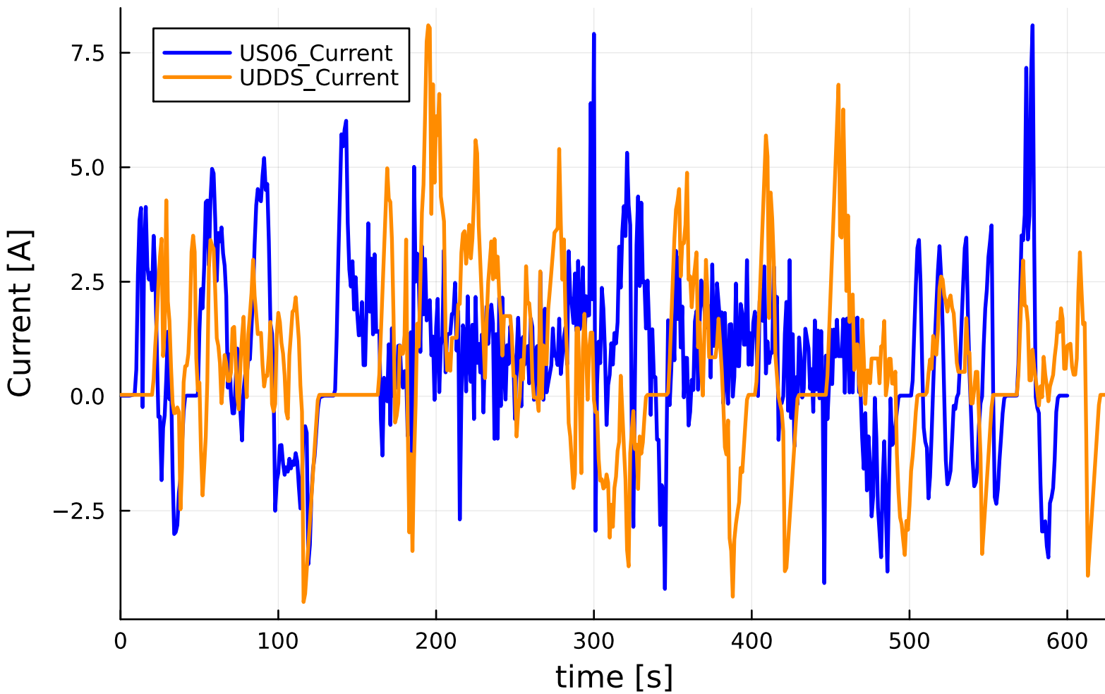
UDDS and US06 Current Profile
