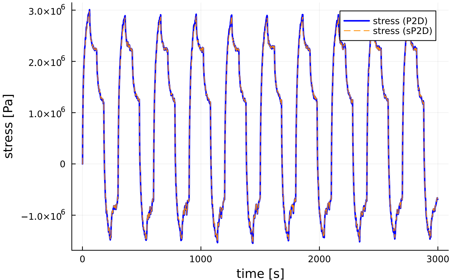
stress_comparison (P2D vs sP2D)
