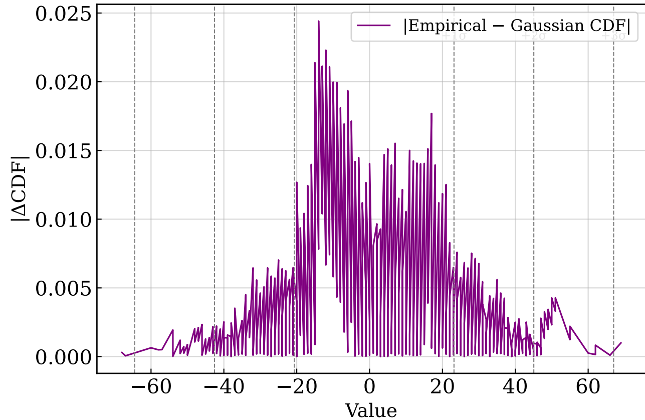
CDF deviation (empirical vs best-fit Gaussian)
