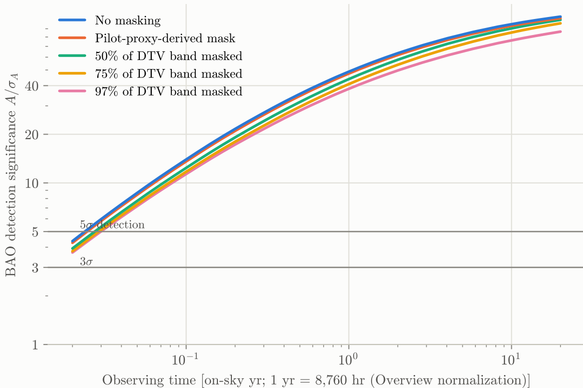
CHIME BAO significance vs observing time under DTV masking
