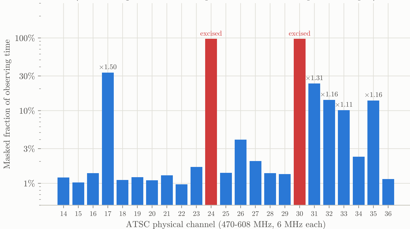
Adopted DTV-channel masking configuration ( \times N = integration-time multiplier to recover clean-equivalent depth)
