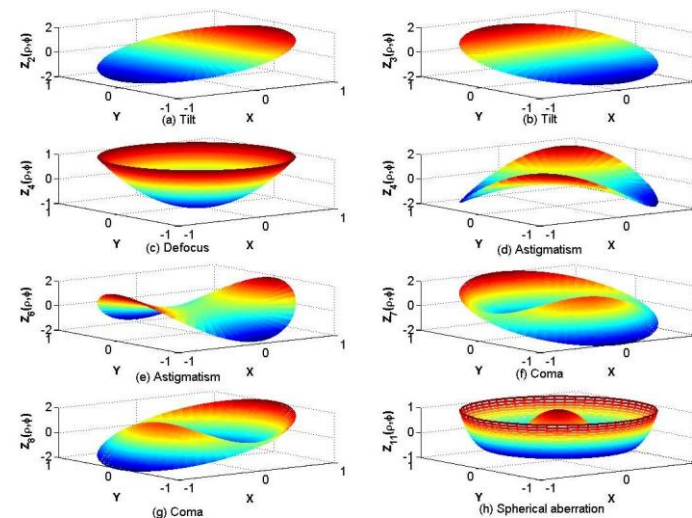
Zernike polynomials
