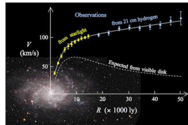
Other galaxy
