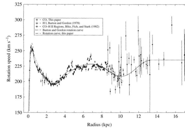
Milky Way
