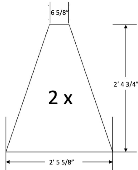
Larger side of horn.
