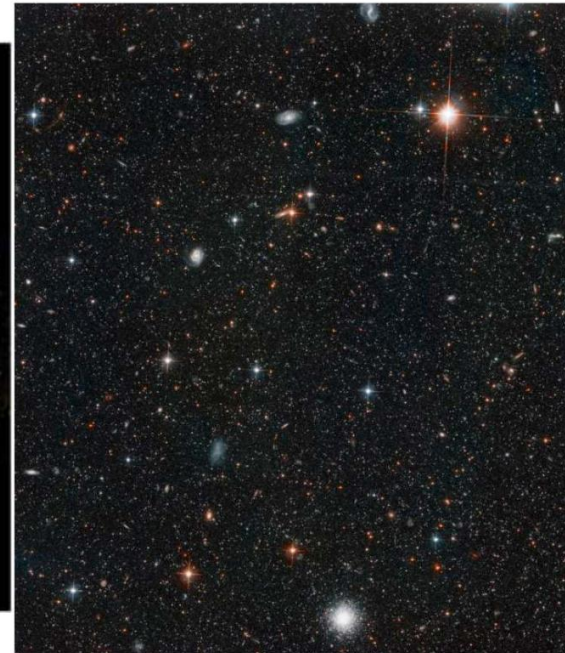
Halo stars
