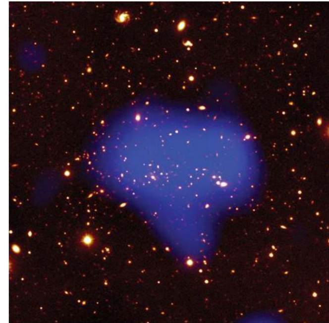
X-rays reveal hot gas between the galaxies.
