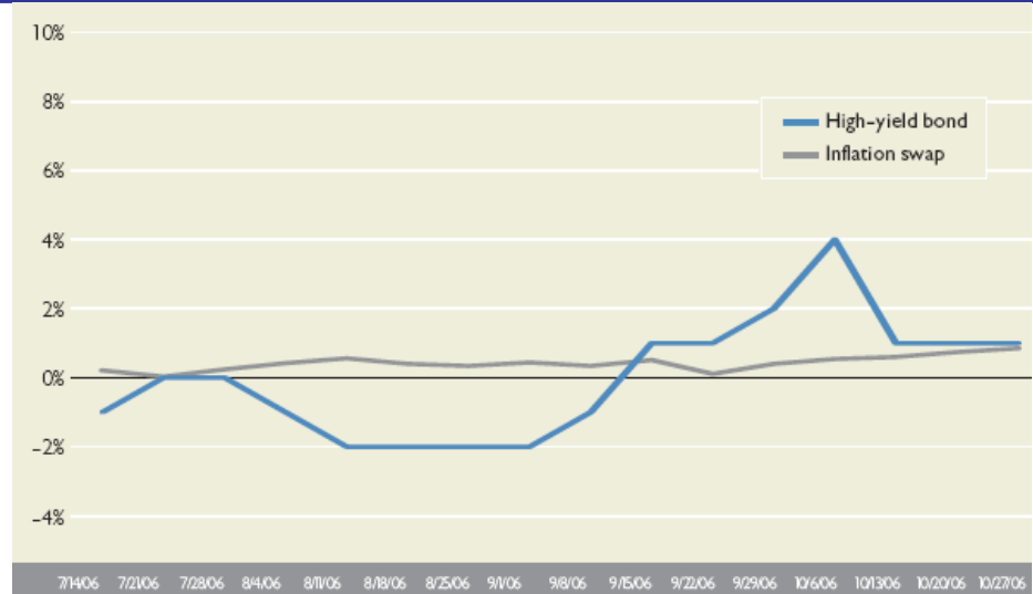
图 5、Inflation SWAPS vs. High-yield Bond Excess Return, (7/14/06–10/27/06)
