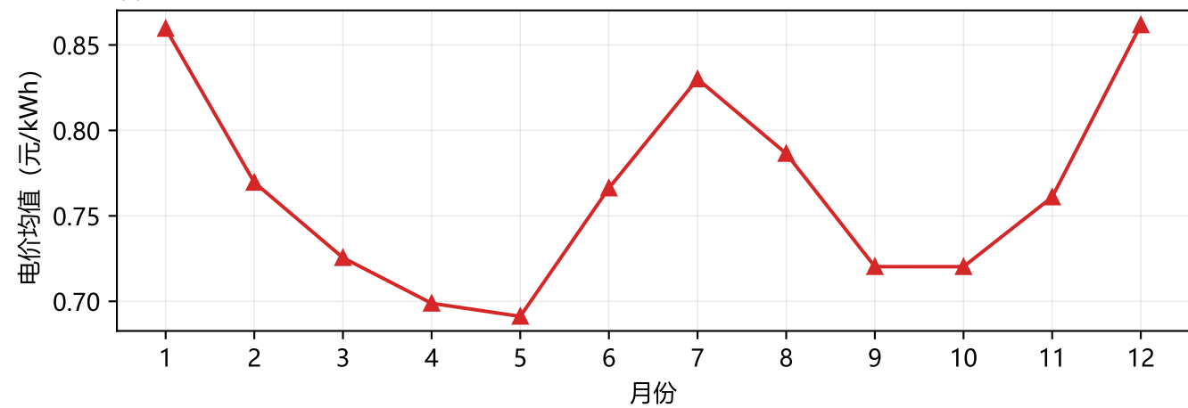
(c) 电价月均值
