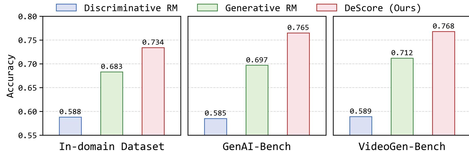
(b) Preference Accuracy
