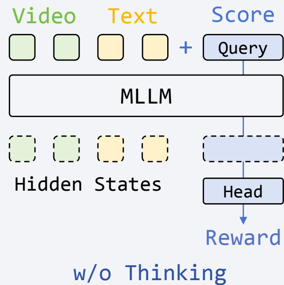
(a) Video Reward Modeling Paradigms
