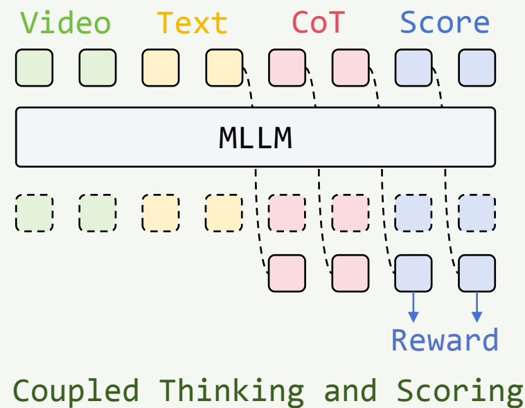
(a) Video Reward Modeling Paradigms
