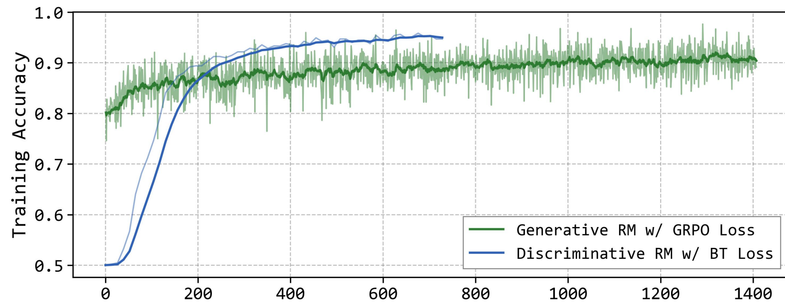
(c) Training Stability
