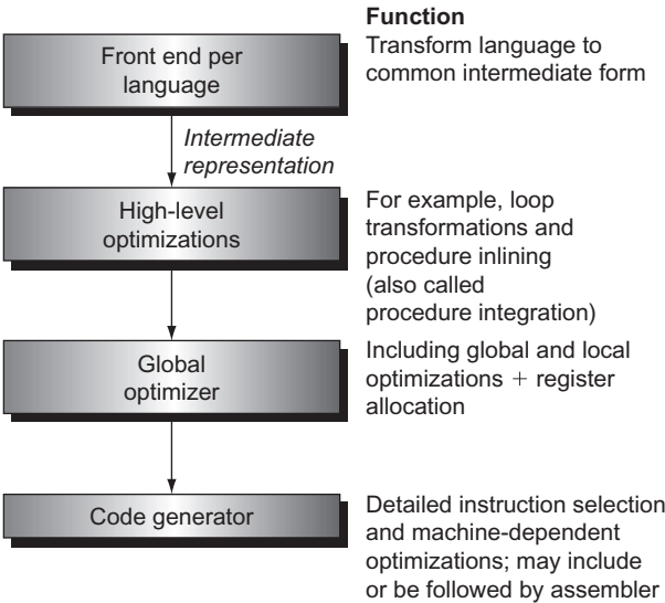
FIGURE e2.15.1 The structure of a modern optimizing compiler consists of a number of passes or phases. Logically, each pass can be thought of as running to completion before the next occurs. In practice, some passes may handle one procedure at a time, essentially interleaving with another pass.
