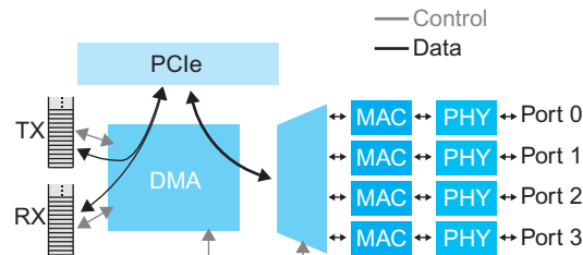
FIGURE e6.9.2 Block diagram of the NetFPGA Ethernet card in Figure e6.9.1 showing the control paths and the data paths. The control path allows the DMA engine to read the status of the queues, such as empty vs. on-empty, and the content of the next available queue entry. The DMA engine also controls port multiplexing. The data path simply passes through the DMA block to the TX/RX queues or to main memory. The “MAC chips” are described below. The PHY chips, which refer to the physical layer, connect the “MAC chips” to physical networking medium, such as copper wire or optical fiber.
