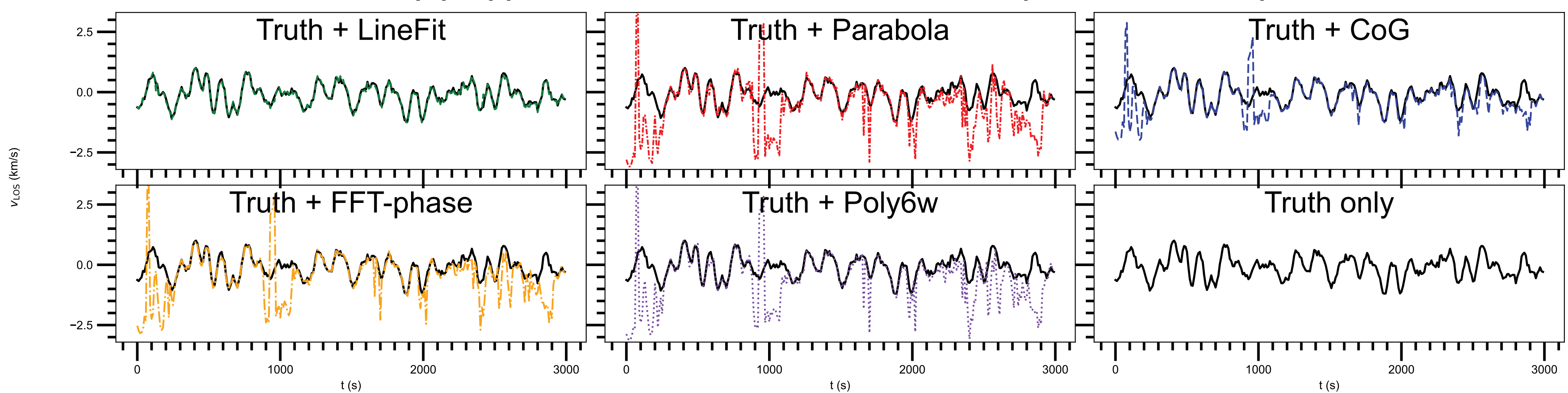
(c) v(t) — multi-lobed/emission line (line number 6)
