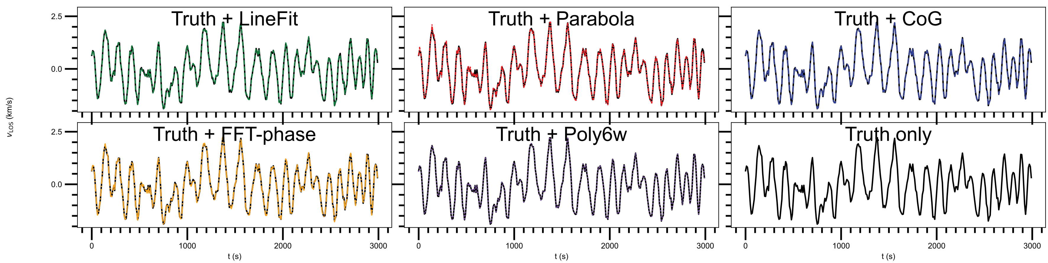
(a) v(t) — isolated symmetric line (line number 1)
