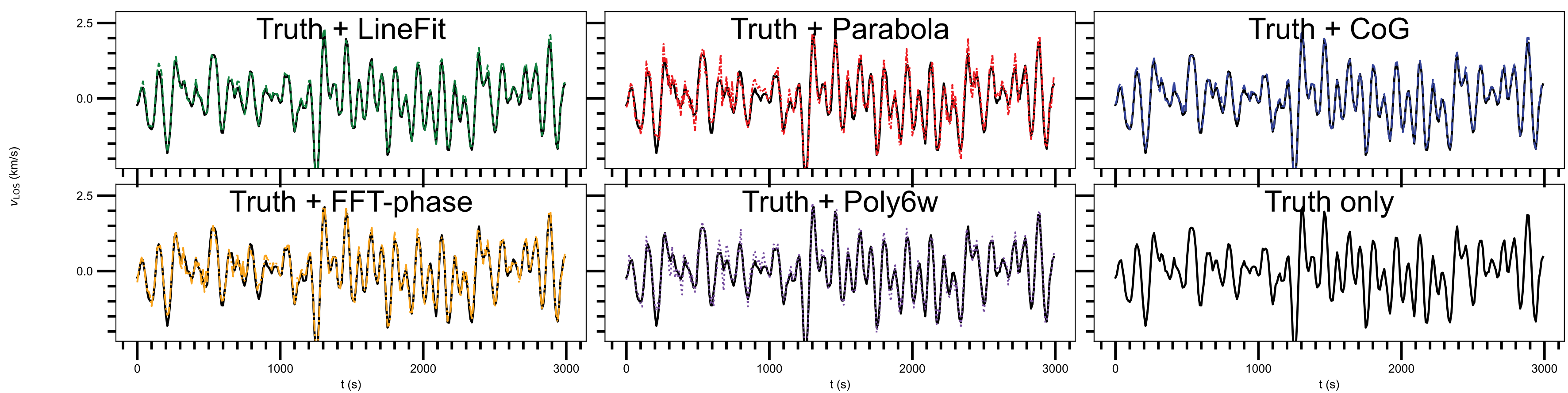
(b) v(t) — blended/asymmetric line (line number 2)
