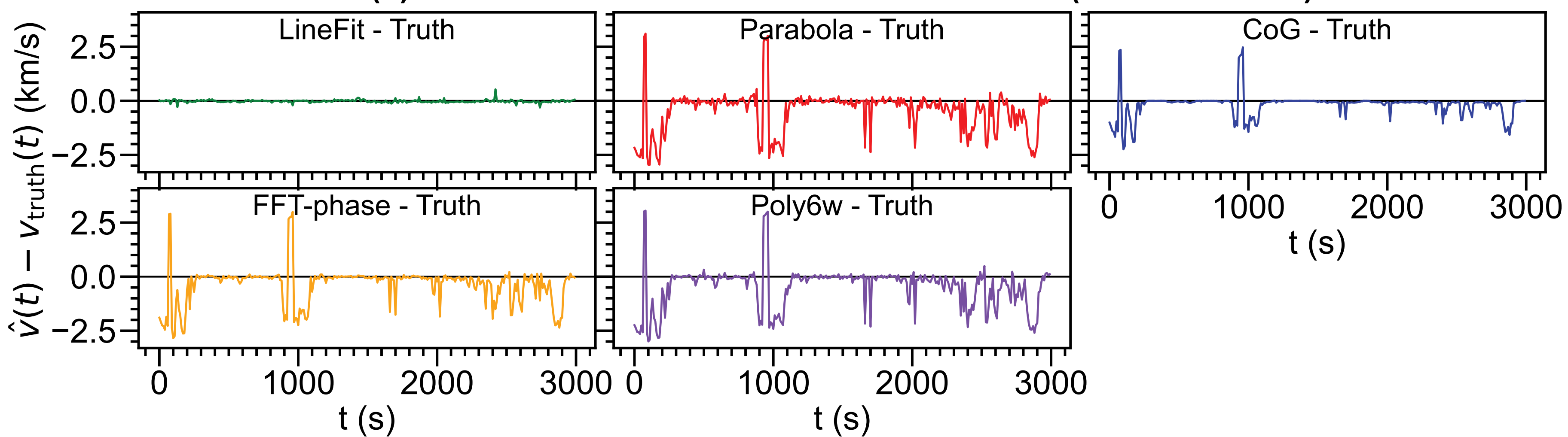
(c) Residuals — multi-lobed/emission line (line number 6)
