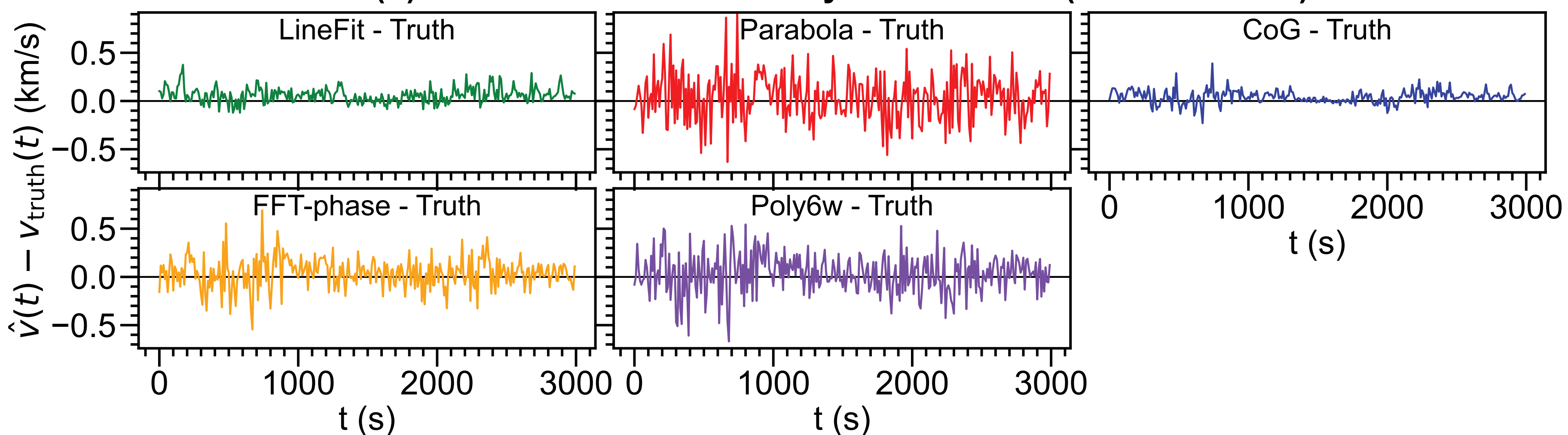
(b) Residuals — blended/asymmetric line (line number 2)
