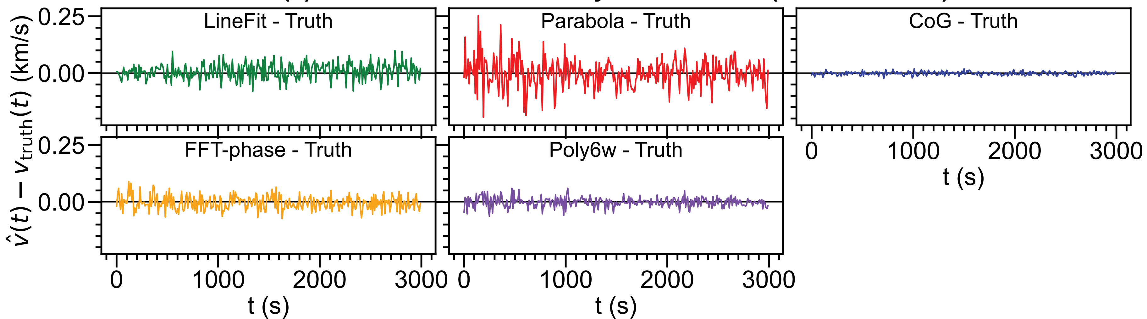
(a) Residuals — isolated symmetric line (line number 1)
