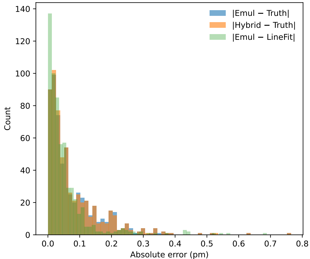
Validation absolute error histograms
