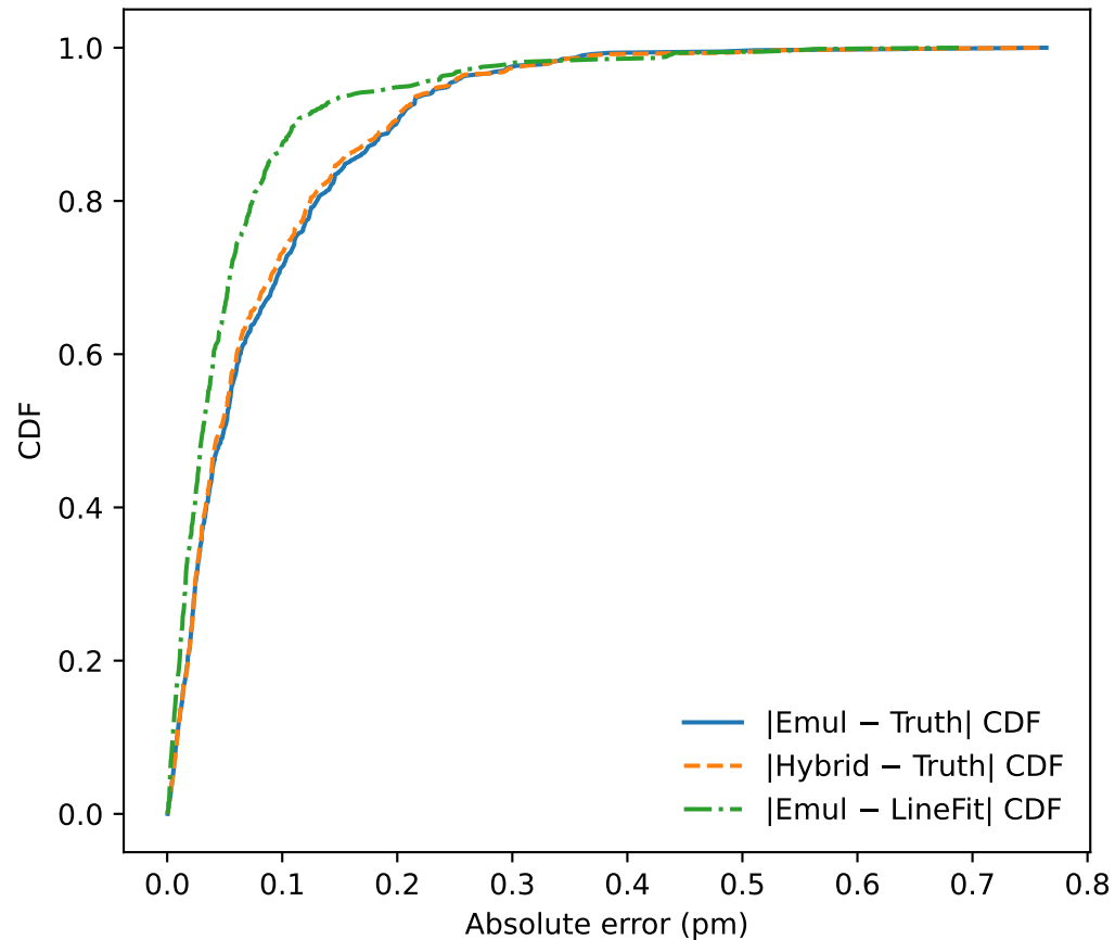
Validation CDFs
