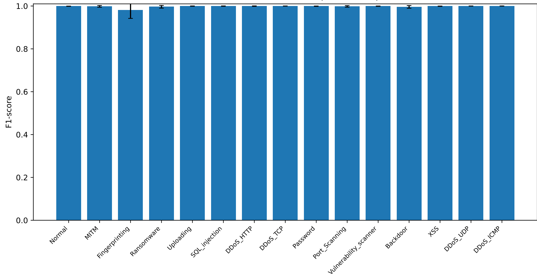
Per-class F1 across 10 folds (mean \pm SD)
