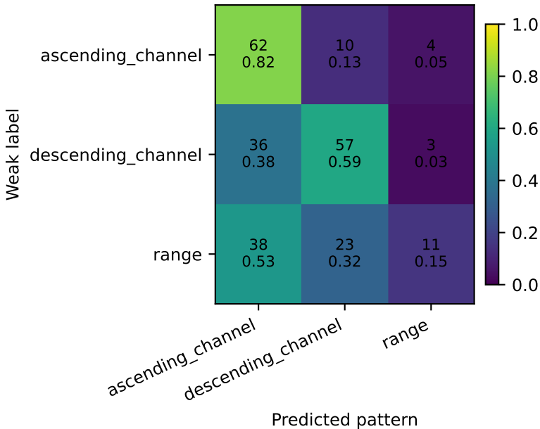
Test confusion matrix (row-normalized)
