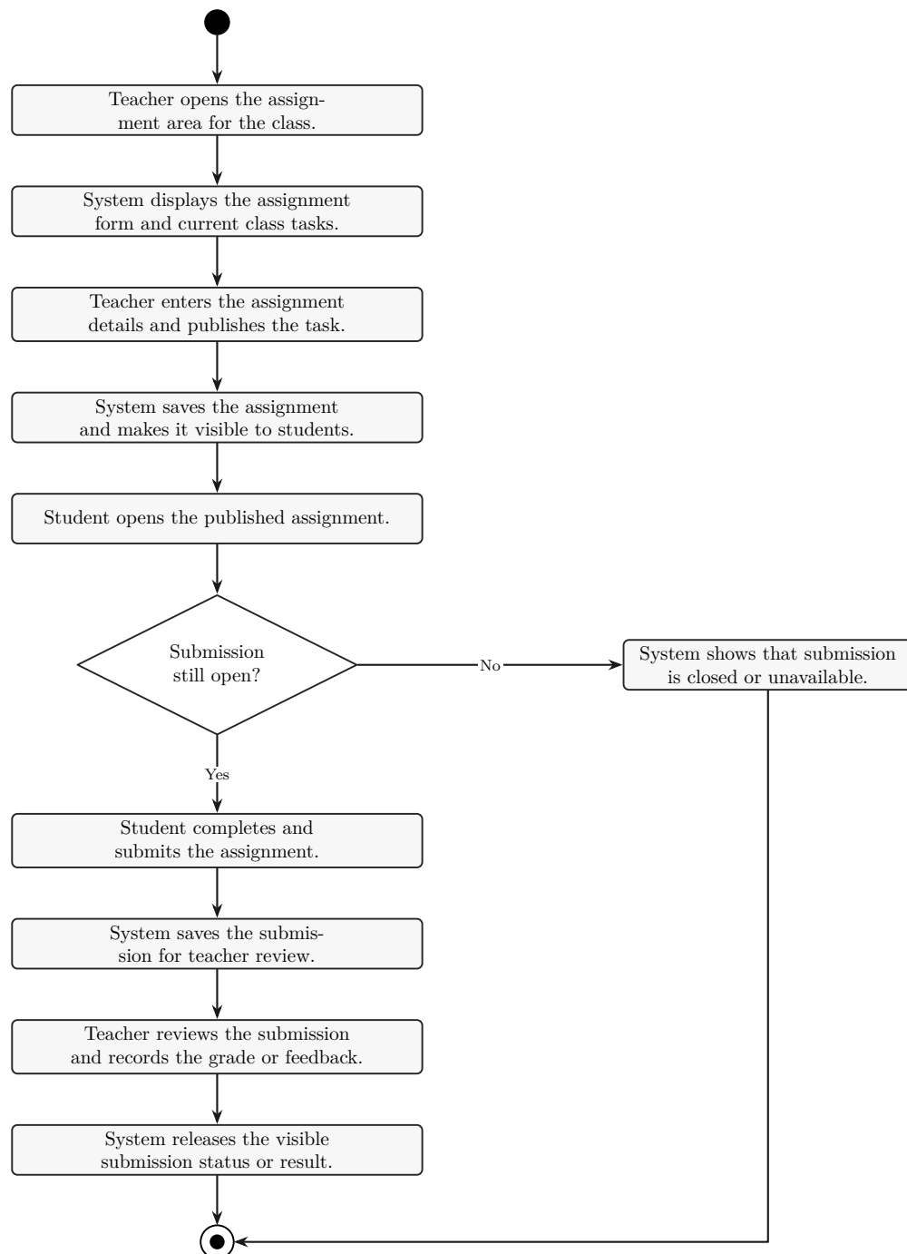
Figure 4.17: Activity diagram representing assignment creation, submission, and grading workflow
