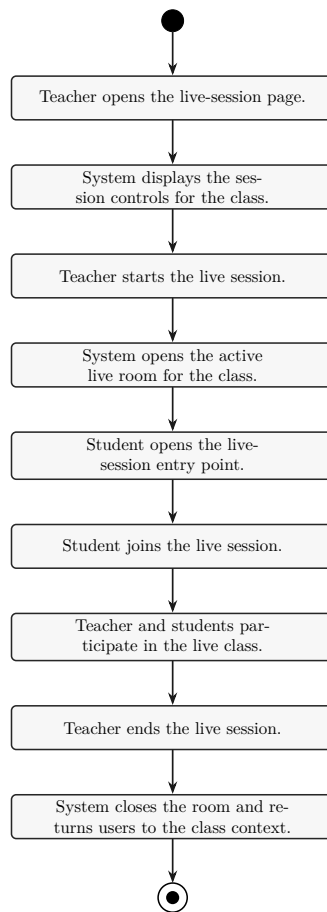
Figure 4.19: Activity diagram representing live session start, join, and end workflow
