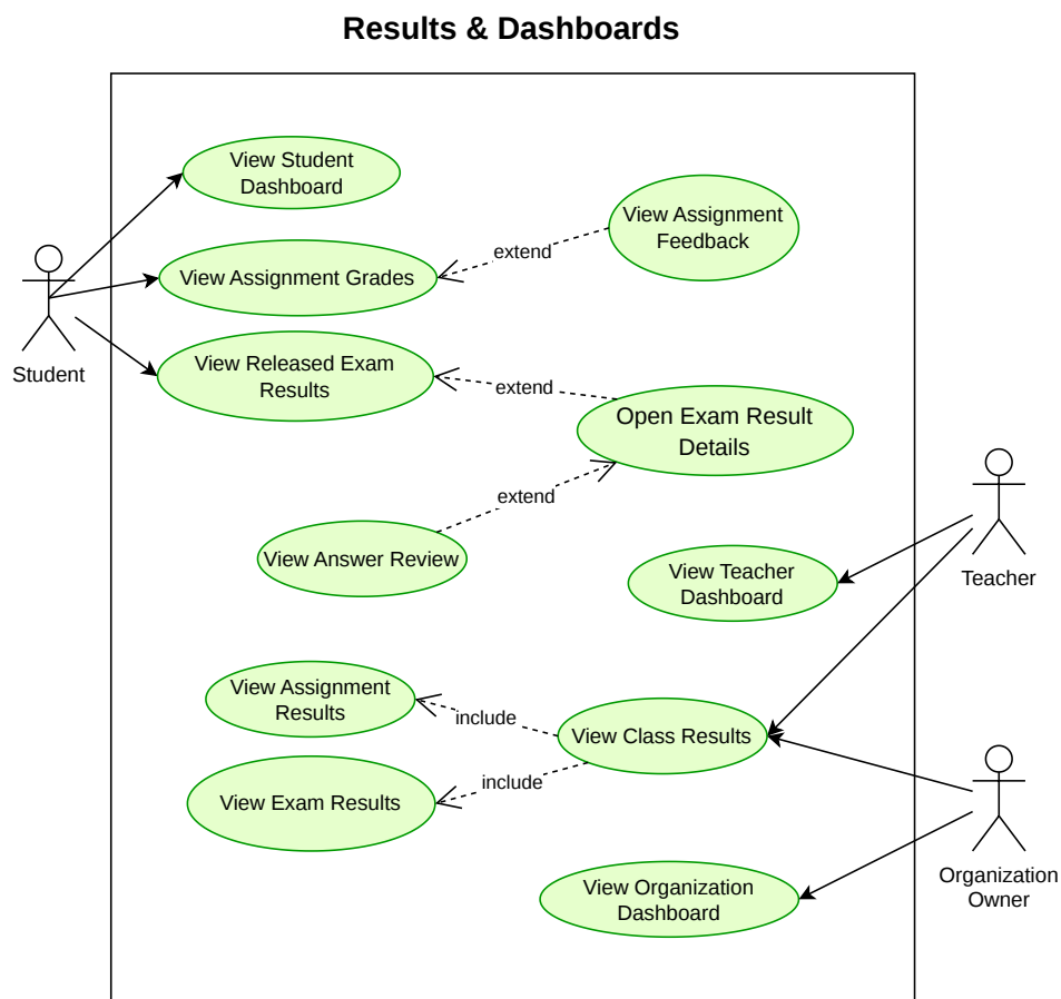
Figure 4.9: Eduverse results and dashboards use-case diagram
