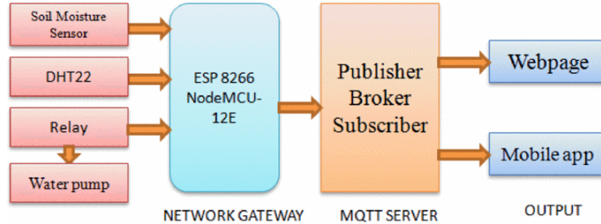
Figure 4.3: Low-cost MQTT-based smart irrigation architecture, adapted from [20]. Source: https://doi.org/10.1109/TENCONSpring.2017.8070095 .
