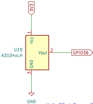
Hall-Effect Sensor (RPM)
