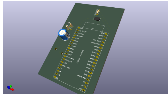
Gambar EL3.7: Tampilan model 3d pcb tampak 3/4
