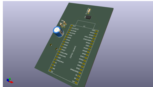
Gambar EL3.13: Tampilan model 3d pcb tampak 3/4
