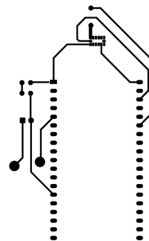
Gambar EL3.11: PCB Mask ISPS
