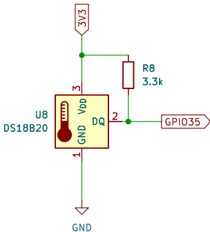
Contact Temperature Sensor
