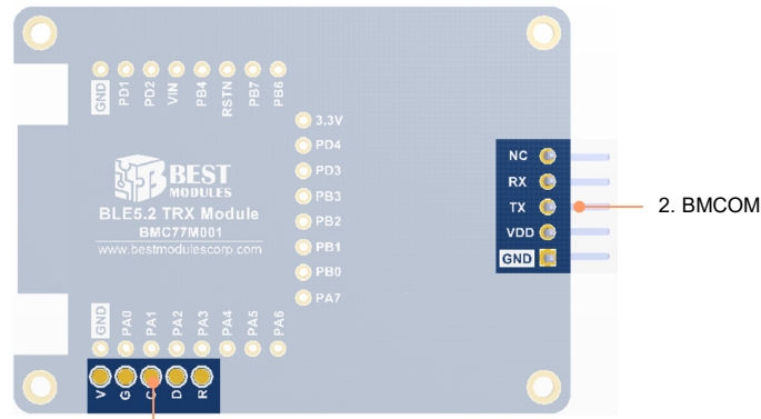
6. Programming Port (Reserved)
