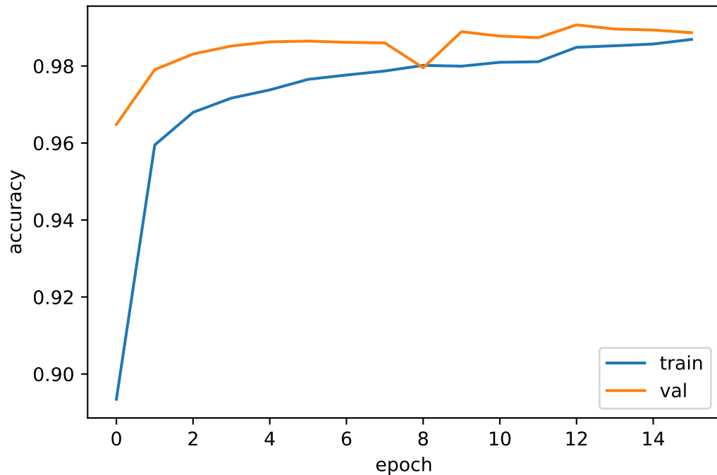
Custom CNN - accuracy
