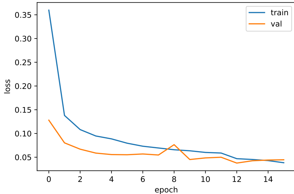
Custom CNN - loss
