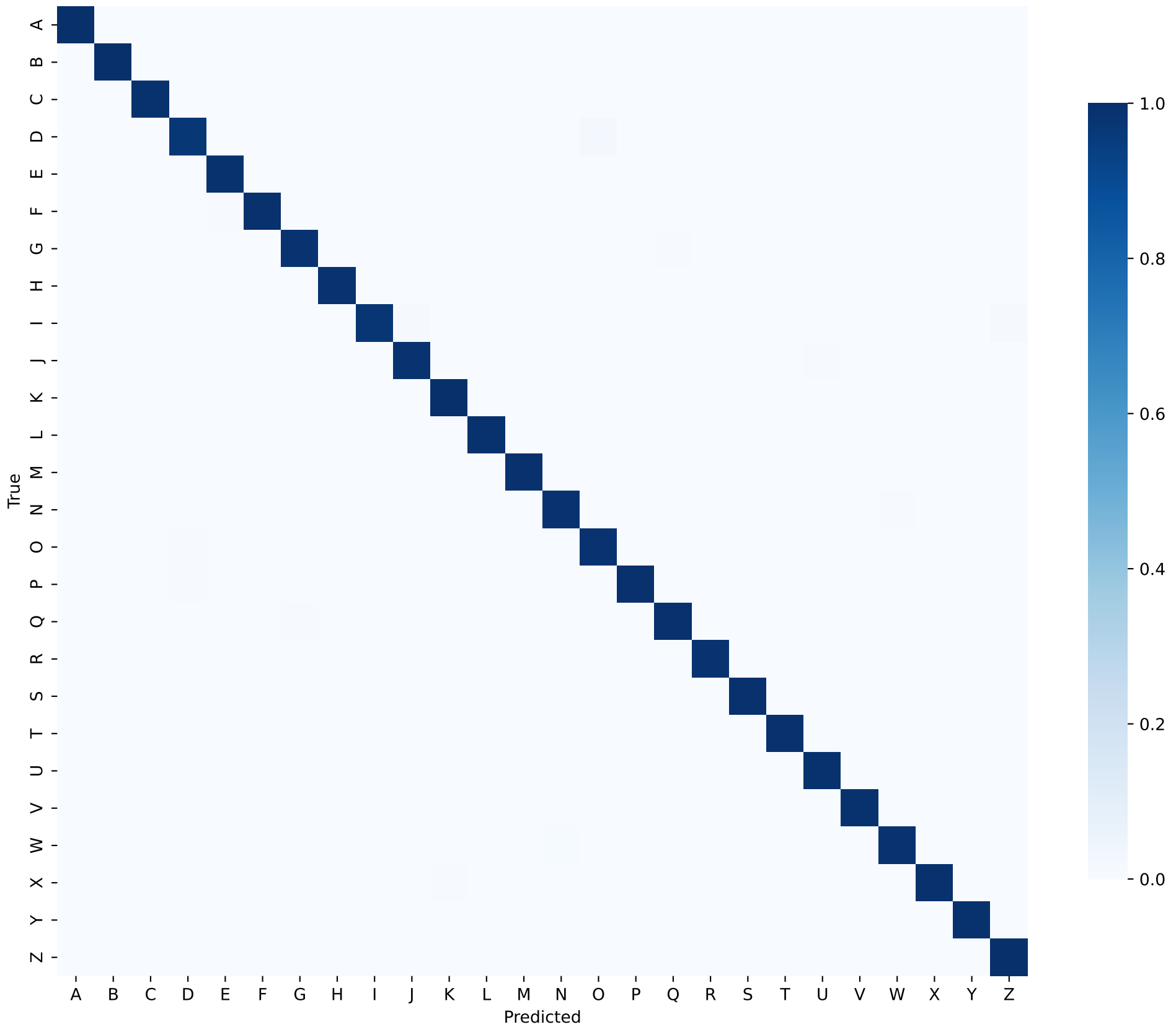
Custom CNN - normalised confusion matrix
