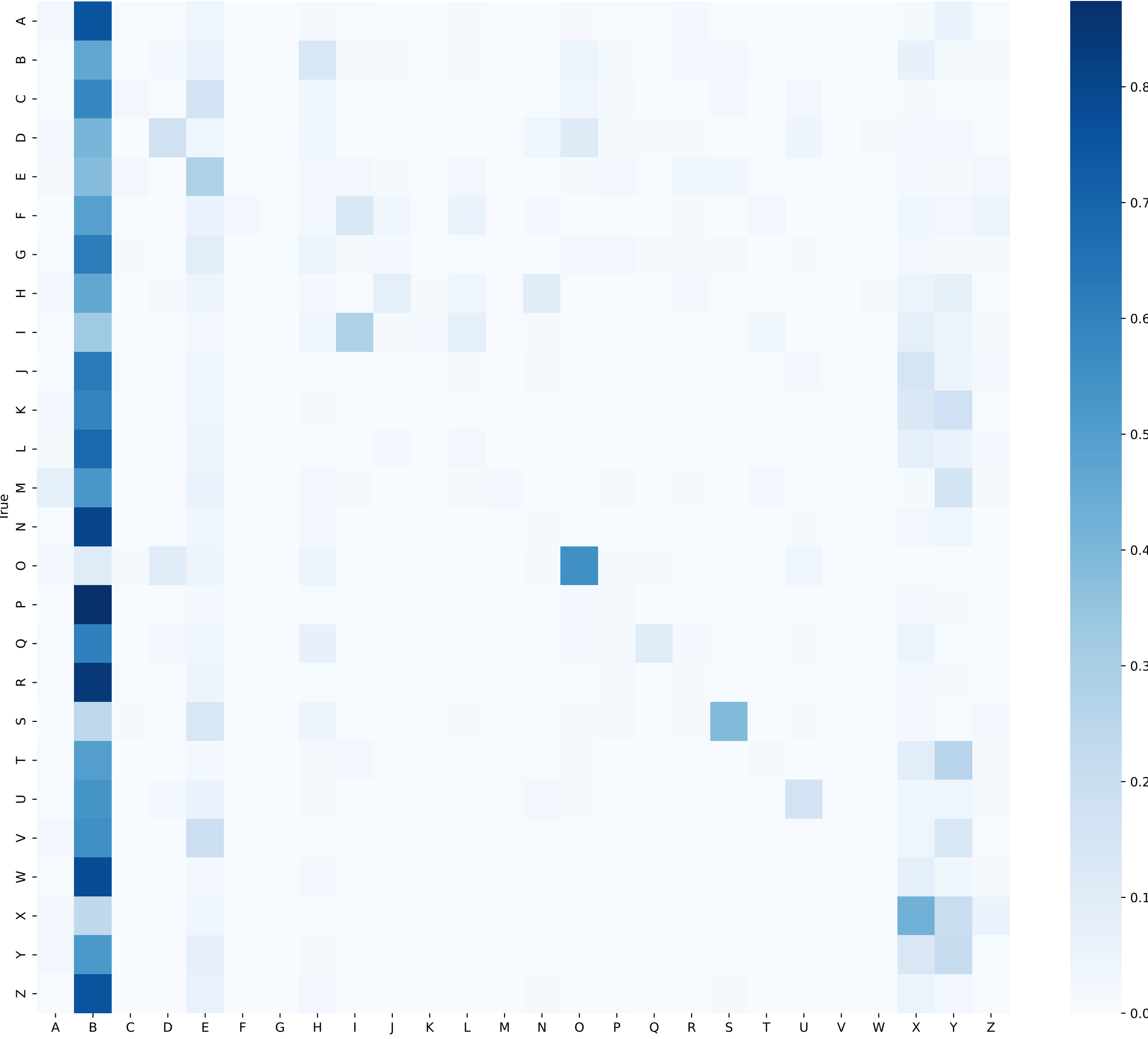
MobileNetV2 — Normalised Confusion Matrix
