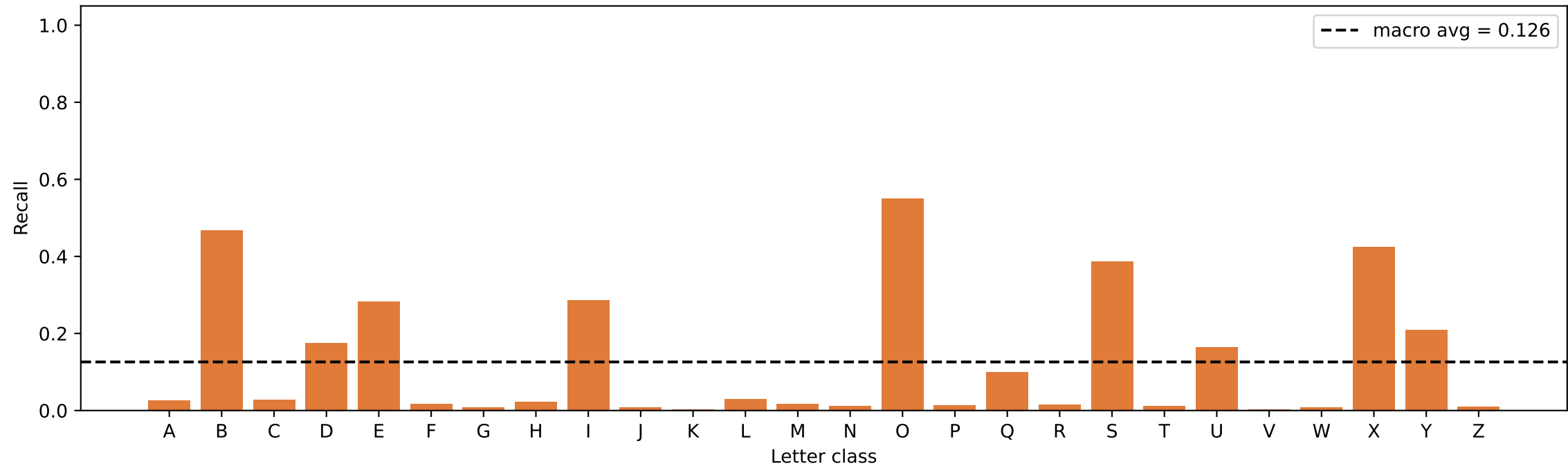
MobileNetV2 — Per-class recall (test set)
