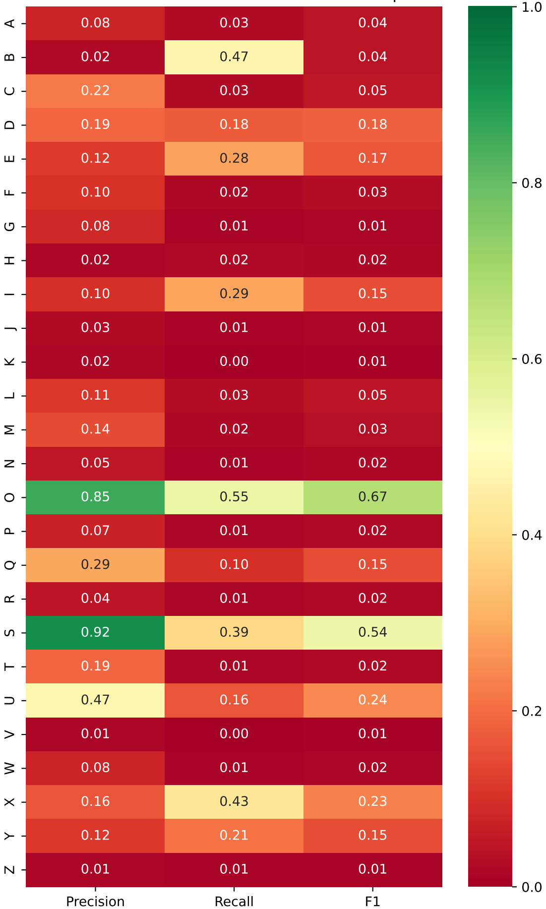
MobileNetV2 — Per-class metrics heatmap
