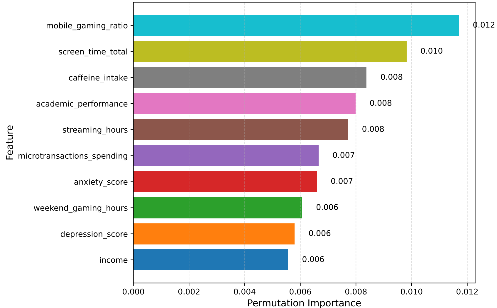
RQ4: Top Features Influencing Mental Health Risk
