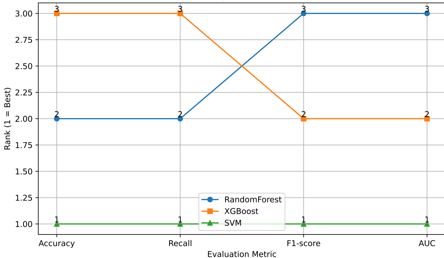
RQ5: Sensitivity to Evaluation Metrics
