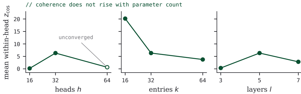
FIGURE 15 · Head coherence against each parameter axis of the star sweep, all runs at 4 epochs (62k steps). No axis delivers the predicted rise; the entries axis falls monotonically. The open marker is the unconverged h=64 run.
