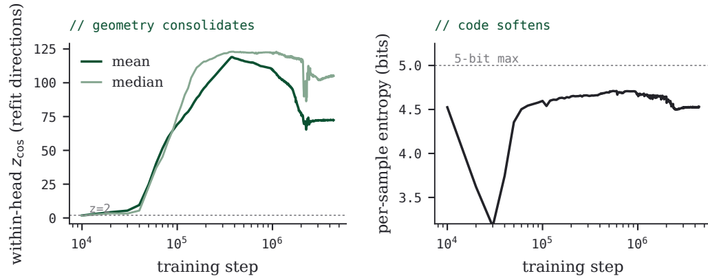
FIGURE 14 · The 448-checkpoint training history of resid_nc_hm . Left: within-head coherence of refit end-to-end directions, z-scored against size-matched nulls; rise, peak near step 370k, partial relaxation. Right: mean per-sample classification entropy returns toward the 5-bit maximum after the annealing transient.
