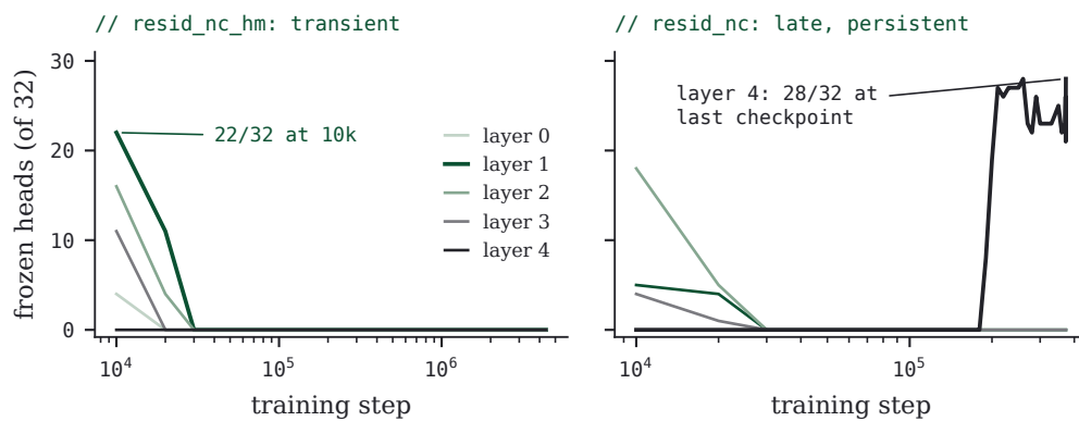
FIGURE 11 · Frozen heads per layer over training. Left: resid_nc_hm , with the mean-entropy bonus, has only an early annealing transient, peaking at 22/32 in layer 1 at step 10k and recovering to zero everywhere by step 30k. Right: resid_nc develops a post-anneal layer-4 freeze from ~190k that persists through its last checkpoint.
