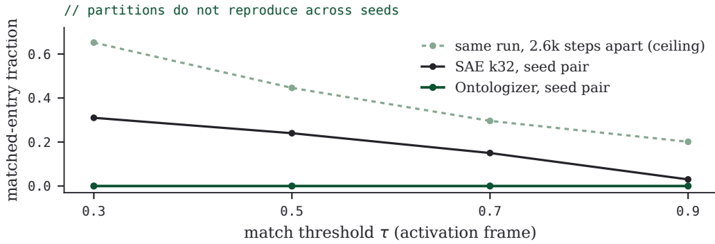
FIGURE 16 · Cross-seed matched-entry fraction on the activation frame by threshold. The same-run pair bounds what the metric can detect (0.65 at \tau=0.3 ); the k32 SAE pair reproduces partially; the softmax Ontologizer’s partitions reproduce not at all.
