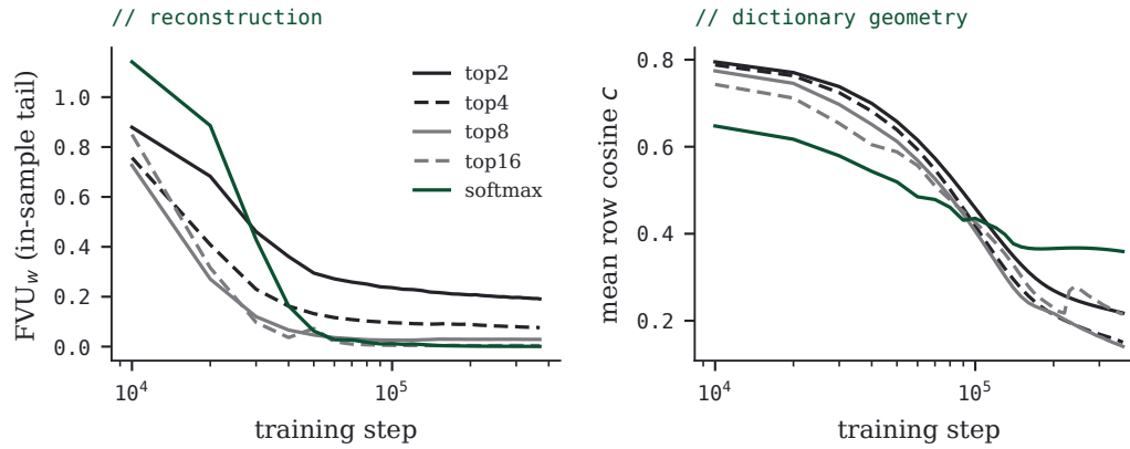
FIGURE 22 · The selection sweep’s _shm arms over training: FVU_w on the (in-sample) tail, scored from each checkpoint, and mean within-head row cosine \bar{\kappa} . The soft arm’s \bar{\kappa} flattens near 0.36 while its error keeps falling; the hard arms keep decorrelating.
