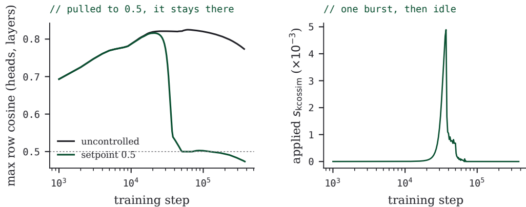
FIGURE 21 · The row-collinearity setpoint on the shipped stack, from the training log. Left: the max within-head row cosine over heads and layers, the statistic the controller watches, against the uncontrolled twin; the dotted line is the 0.5 setpoint. Right: the applied multiplier s_{kcossim} , averaged over 1000-step windows.
