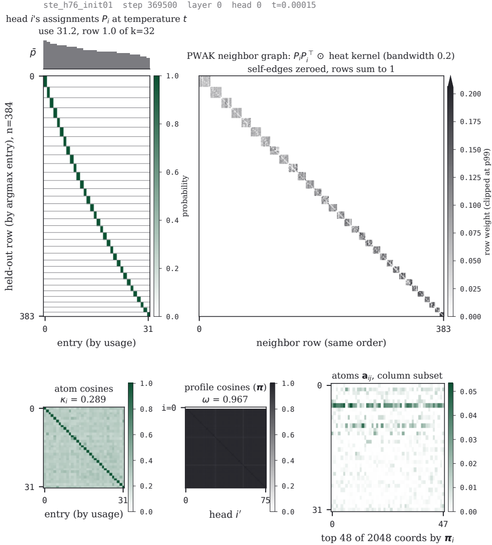
FIGURE 4 · One trained head, block by block. Head i=0 of layer 0 of the straight-through model ste_h76_init01 (step 369,500, t=0.00015 ) on n=384 rows drawn from the eval tail; one seed. Top left: the assignments P_i , rows sorted by winning entry and entries by mean usage \bar{p}_{ij} (bars). “Use” is the effective number of entries across rows, \exp H(\bar{\mathbf{p}}_i) , and “row” the effective number within a row, the exponential of the mean per-row entropy: 31.2 and 1.0 of k=32 , a hard code that uses nearly every entry. Top right: the neighbor graph that \text{KL}_{\text{pwak}} and \text{L2}_{\text{pwak}} (Eq. (22)) diffuse over, in the same row order: the co-assignment matrix P_i P_i^\top times the heat kernel \exp((\langle \mathbf{u}_n, \mathbf{u}_{n'} \rangle - 1)/0.2) of the layer’s shapes without their constant coordinate, self-edges removed and each row normalized to sum to one. A hard code makes it block-diagonal by cell. This model was not trained with either statistic, so the graph is the one they would build, not one that shaped it. Bottom: cosines between head i ’s atoms, whose off-diagonal mean is \kappa_i (0.289); cosines between the heads’ coordinate profiles \pi (Eq. (6)) with \bar{\mathbf{p}} the mean over the n rows, whose off-diagonal mean is \omega (0.967), head i ’s row outlined; and head i ’s atoms on the 48 of e=2048 coordinates where \pi_i is largest, a column subset rather than a projection. Each block has its own scale, white at zero. Figure 10 is the same head of a softmax model.
