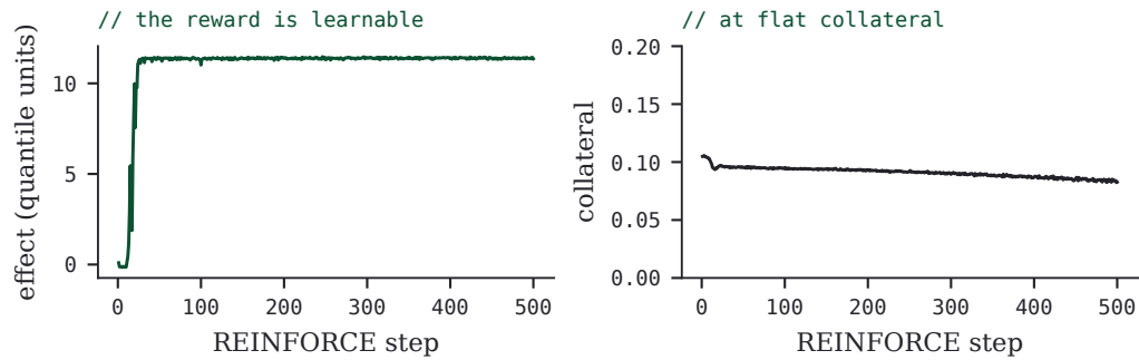
FIGURE 18 · REINFORCE against a single frozen classification's quantile-normalized score, in-embedding tier. The policy saturates the reward within roughly 40 steps while collateral stays at its starting level.
