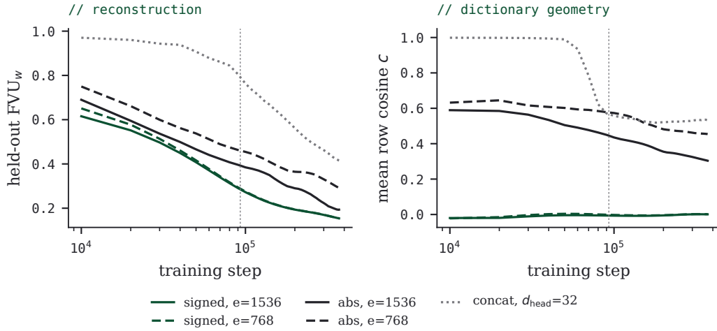
FIGURE 8 · The orthant arms over training: held-out FVU_w scored from each checkpoint (left) and mean within-head row cosine (right). The dotted line marks step 90k. The signed arms coincide at both widths; abs is behind at both, and further behind at the square decoder.
