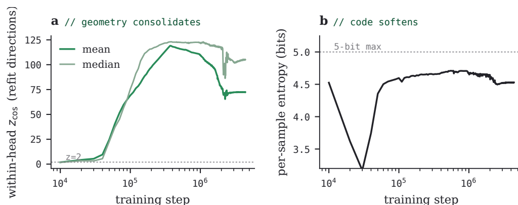
FIGURE 22 · The 448-checkpoint training history of resid_nc_hm . (a) Within-head coherence of refit end-to-end directions, z-scored against size-matched nulls; rise, peak near step 370k, partial relaxation. (b) Mean per-sample classification entropy returns toward the 5-bit maximum after the annealing transient.
