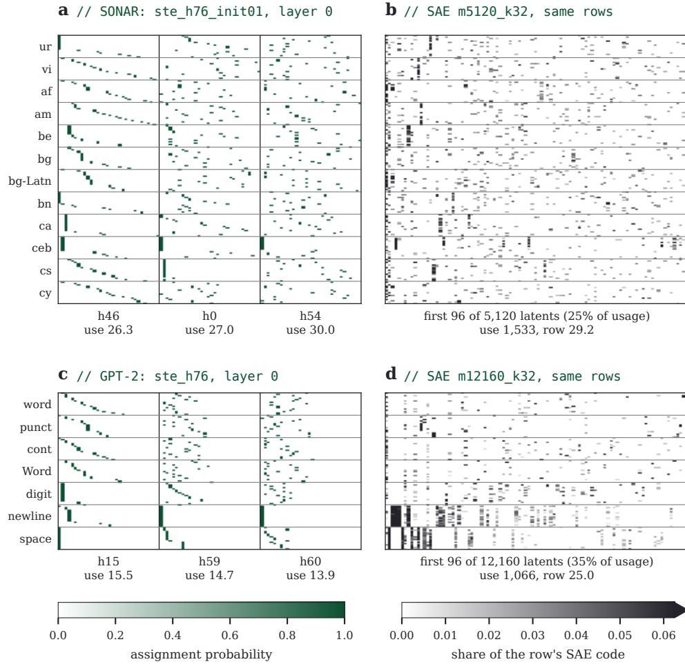
FIGURE 16 · Hard codes against SAE codes, row by row. Layer-0 assignments of the straight-through stacks on eval-tail rows, 24 per label value: (a) SONAR ste_h76_init01 by language, (c) GPT-2 ste_h76 by token class, for the three heads whose partitions carry the most NMI with the label above its shuffled null. Entries are sorted by usage, rows grouped by label and ordered by their winning entries; each head's use is under it, and its row is 1.0. (b, d) The same rows in the same order against an SAE trained on the same cache (m5120_k32, m12160_k32), each cell a latent's share of the row's code, for the 96 latents most used on these rows; the whole code's use and row are under it. One seed per model.
