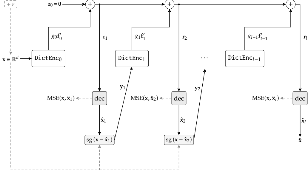
FIGURE 2 · Ontologizer architecture. Each DictEnc writes its gain-scaled output g_\ell f'_\ell into a shared accumulator. States count the layers applied: layer \ell reads r_\ell and the residual y_\ell , and writes r_{\ell+1} . One decoder serves every prefix, and each prefix is scored against x (deep supervision). The dashed input-noise hook is off in every reported model. Section 3.1.5 gives the equations.
