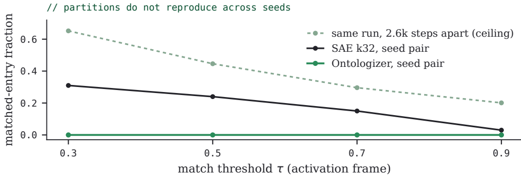
FIGURE 25 · Cross-seed matched-entry fraction on the activation frame by threshold. The same-run pair bounds what the metric can detect (0.65 at \tau=0.3 ); the k32 SAE pair reproduces partially; the softmax Ontologizer’s partitions reproduce not at all.
