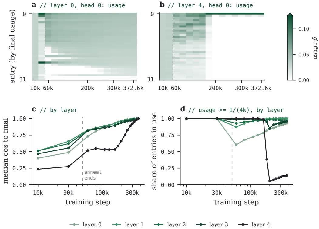
FIGURE 23 · Entries settle after the anneal. resid_nc's 16 retained checkpoints on the eval tail. (a, b) Usage \bar{p}_{ij} of head 0's 32 entries in layers 0 and 4, one column per checkpoint (not to scale in step), entries ordered by final usage; the dotted line marks the anneal's end. (c) Per layer, the median cosine between an entry's decoded atom and its final direction, over the entries in use at the last checkpoint. (d) Per layer, the share of entries in use ( \bar{p}_{ij} \geq 1/(4k) ). One seed.
