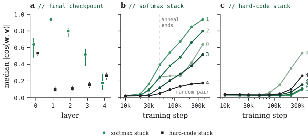
FIGURE 34 · The softmax stack’s classifier features go rank 1; the hard-code stack’s mostly do not. Median |\cos \angle(\mathbf{w}, \mathbf{v})| of each layer’s bilinear feature pairs (bilinspec.py), 1 for a rank-1 feature. (a) The final checkpoint by layer, with interquartile ranges: the softmax stack (resid_nc, step 372.6k) and the hard-code stack (ste_h76_init01, step 369.5k). (b, c) Over training, one line per layer, numbered at its end; the softmax stack’s temperature anneal ends at 50k, and the hard-code stack’s temperature is constant. Dashed: the median for a random pair in the 1024-dimensional semantic block, 0.021. One seed per run.
