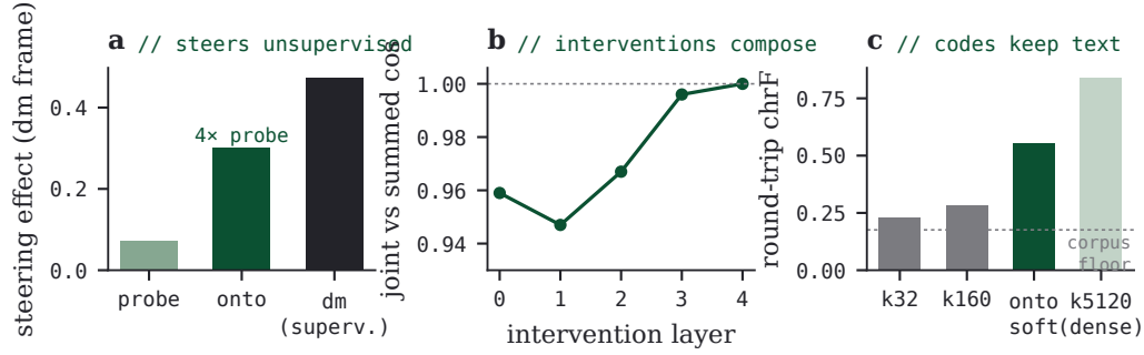
FIGURE 1 · The softmax Ontologizer’s steering primitive, measured. (a) Forcing an entry moves decodes along the supervised difference-of-means direction 0.64\times as far as supervised steering itself and 4\times as far as probe directions ( resid_nc_hm ; Table 17). (b) Joint two-head interventions point where the summed single interventions point, exactly in the final layer ( resid_nc ; Section 8). (c) The sparse SAEs’ codes lose most text before any intervention (round-trip chrF 0.23–0.28 against a 0.18 corpus floor) while the soft code keeps it (0.55); the dense k5120 keeps more but is not a sparse code (Appendix C.5).
