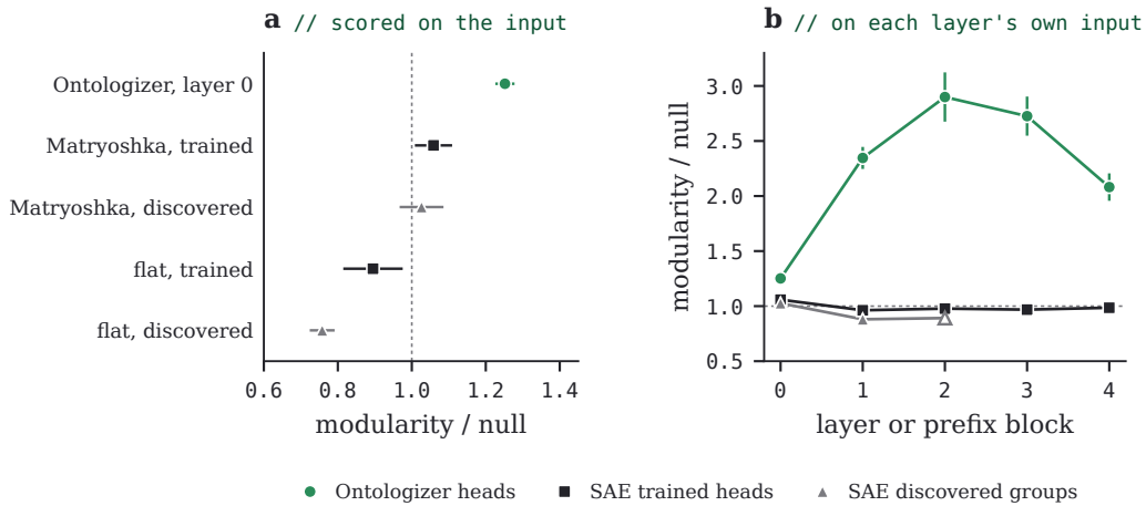
FIGURE 17 · Ontologizer heads are communities of the residual they classify; SAE heads and groups are not. Soft modularity over its size-matched null ( headstruct.py -modularity, Eq. (34)); bars are \pm 2 null standard deviations. (a) Every model scored on the input itself: the softmax Ontologizer’s layer 0, block 0 of the two Matryoshka SAEs (scored on \mathbf{x} - \mathbf{b}_{\text{dec}} , the SAE encoder’s input), and the two flat SAEs. (b) By depth, each layer or prefix block on the graph of its own input. Hollow: a block whose groups cover under 10% of samples. The discovered groups’ blocks 3 and 4 are not drawn: block 3’s null is within two of its standard deviations of 0 (3% coverage), and block 4 holds one group, which its null reproduces exactly. One checkpoint per model.
