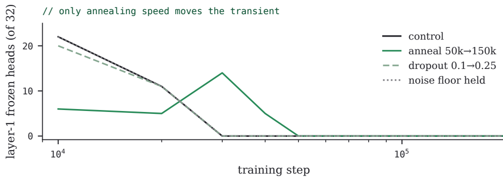
FIGURE 20 · The early transient under the four retrains, layer-1 frozen count. The noise-floor variant overlaps the control exactly and the dropout variant tracks it to within two heads at the peak; only stretching the temperature anneal moves the curve, trading peak height for duration.
