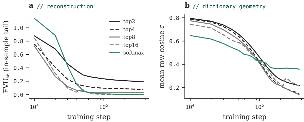
FIGURE 32 · The selection sweep’s _shm arms over training: (a) FVU_w on the (in-sample) tail, scored from each checkpoint, and (b) mean within-head row cosine \bar{\kappa} . The soft arm’s \bar{\kappa} flattens near 0.36 while its error keeps falling; the hard arms keep decorrelating.
