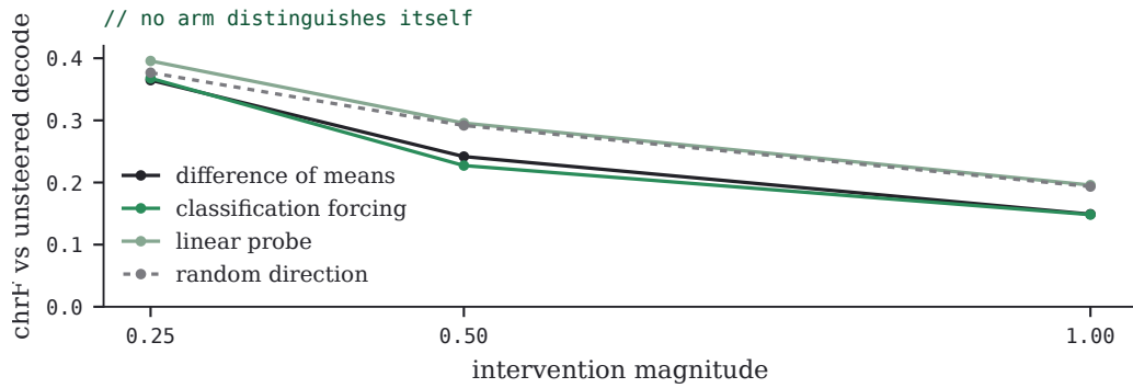
FIGURE 26 · chrF between steered and unsteered decodes by intervention magnitude. All four arms, the random direction included, damage the decode at nearly the same rate; no arm buys naturalness at matched magnitude.
