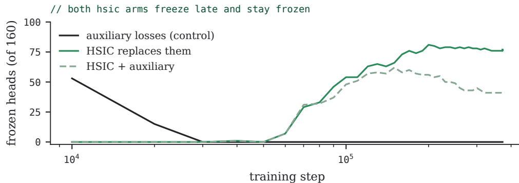
FIGURE 21 · Total frozen heads over training for the three loss configurations, all on the resid_nc_hm configuration at 372k steps. The auxiliary-loss control’s freeze is the early transient and resolves; both HSIC arms, whose head-CKA penalty uses the biased estimator, develop the late, persistent freeze instead, and the auxiliary terms only partially thaw it.
