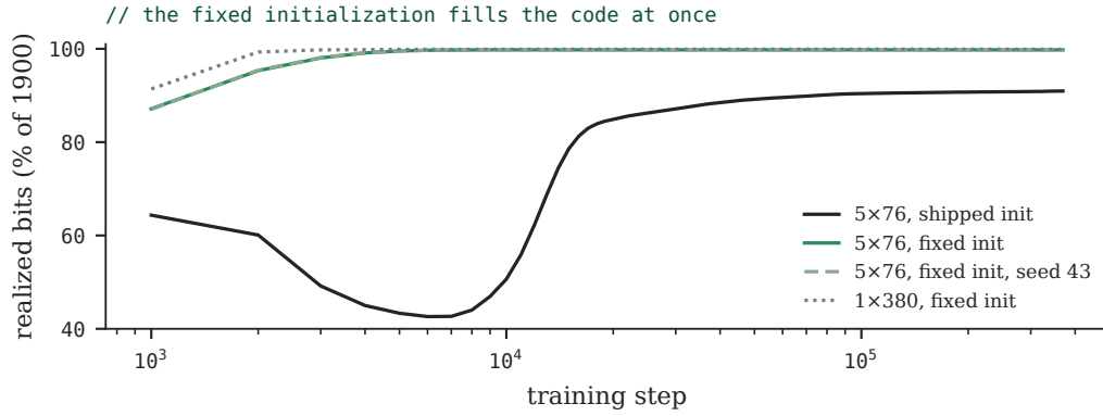
FIGURE 28 · Realized code bits over training, as a share of the nominal 1900, from the logged KL_m less its one-batch sampling floor. The shipped initialization’s head usage collapses to under half before recovering to 90% (the curve’s 91% over-corrects heads with dead entries); at the fixed initialization every head in the stack and the flat arm reaches near-uniform usage within 5k steps. An upper bound on the information carried, not a measure of it (Eq. (35)).
