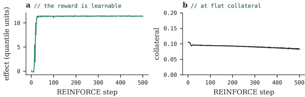
FIGURE 27 · REINFORCE against a single frozen classification’s quantile-normalized score, in-embedding tier. The policy saturates the reward within roughly 40 steps (a) while collateral stays at its starting level (b).
