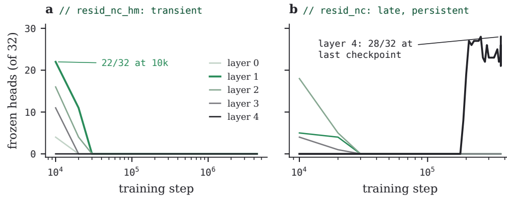
FIGURE 19 · Frozen heads per layer over training. (a) resid_nc_hm , with the mean-entropy bonus, has only an early annealing transient, peaking at 22/32 in layer 1 at step 10k and recovering to zero everywhere by step 30k. (b) resid_nc develops a post-anneal layer-4 freeze from ~190k that persists through its last checkpoint.
