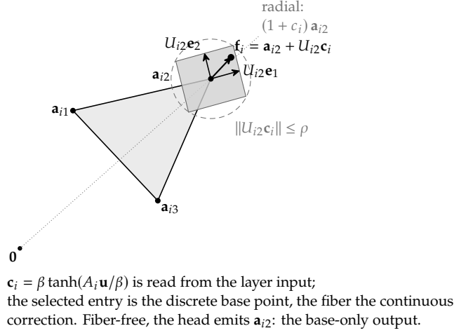
FIGURE 7 · Fiber geometry for one head, extending Figure 5. The head selects the entry with atom \mathbf{a}_{i2} ; its fiber is the plane spanned by U_{i2} at that point, and the coordinates \mathbf{c}_i place the output within it. The dashed circle is the per-head norm cap; the dotted ray is the radial variant, which moves the output only along the atom’s own direction.
