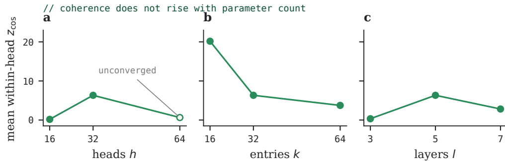
FIGURE 24 · Head coherence against each parameter axis of the star sweep: heads (a), entries (b) and layers (c), all runs at 4 epochs (62k steps). No axis delivers the predicted rise; the entries axis falls monotonically. The open marker in (a) is the unconverged h=64 run.
