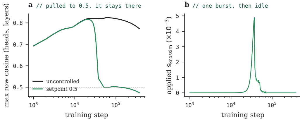
FIGURE 31 · The row-collinearity setpoint on the shipped stack, from the training log. (a) The max within-head row cosine over heads and layers, the statistic the controller watches, against the uncontrolled twin; the dotted line is the 0.5 setpoint. (b) The applied multiplier s_{kcosim} , averaged over 1000-step windows.
