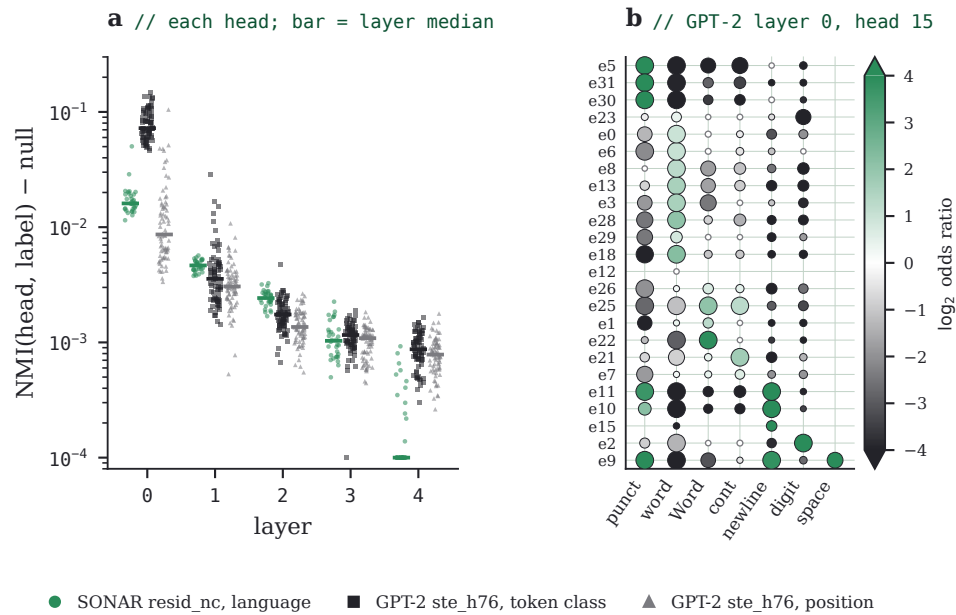
FIGURE 18 · Label structure lives in layer 0. (a) NMI between each head's winning entry and a label on the eval tail, less its mean over five label-shuffled draws, one point per head (values at or below that mean drawn at 10^{-4} ) and a bar at the layer median: resid_nc against language, GPT-2 ste_h76 against token class and position. (b) The GPT-2 layer-0 head with the most token-class NMI (head 15), each entry against each class: colour the Haldane-corrected \log_2 odds ratio, area -\log_{10} FDR (capped at 50), filled where FDR < 0.05 ; entries grouped by the class they are most enriched for. One seed per model.
