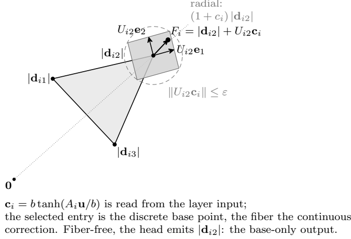
Figure 5: Fiber geometry for one head, extending Figure 3. The head selects entry |\mathbf{d}_{i2}| ; its fiber is the plane spanned by U_{i2} at that point, and the coordinates \mathbf{c}_i place the output within it. The dashed circle is the per-head norm cap; the dotted ray is the radial variant, which moves the output only along the entry’s own direction.
