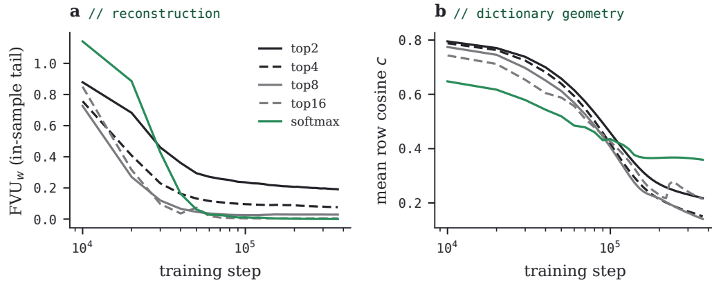
FIGURE 32 · The selection sweep’s _shm arms over training: (a) FVU_w on the (in-sample) tail, scored from each checkpoint, and (b) mean within-head row cosine \bar{c} . The soft arm’s \bar{c} flattens near 0.36 while its error keeps falling; the hard arms keep decorrelating.
