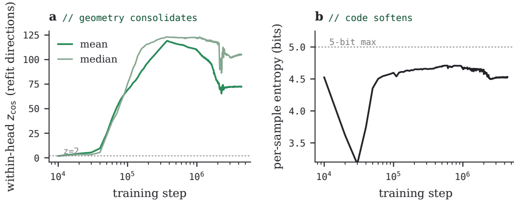
FIGURE 22 · The 448-checkpoint training history of resid_nc_hm. (a) Within-head coherence of refit end-to-end directions, z-scored against size-matched nulls; rise, peak near step 370k, partial relaxation. (b) Mean per-sample classification entropy returns toward the 5-bit maximum after the annealing transient.
