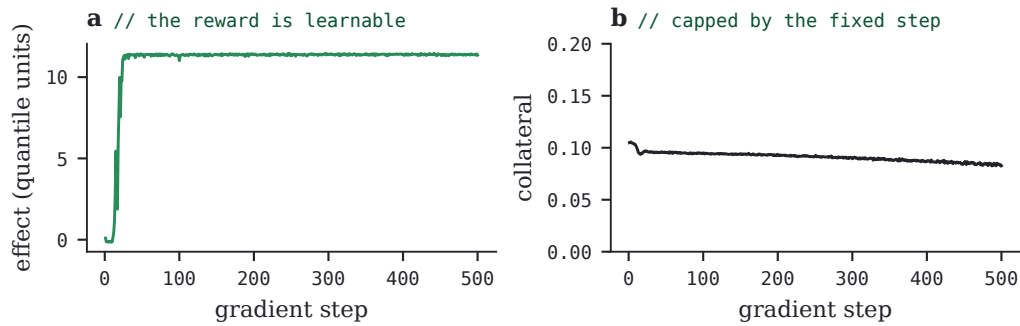
FIGURE 27 · A steering policy trained by gradient ascent on a single frozen classification’s quantile-normalized score, in-embedding tier. The policy saturates the reward within roughly 40 steps (a); collateral, capped at 0.134 by the fixed step length, falls from 0.105 to 0.083 (b).
