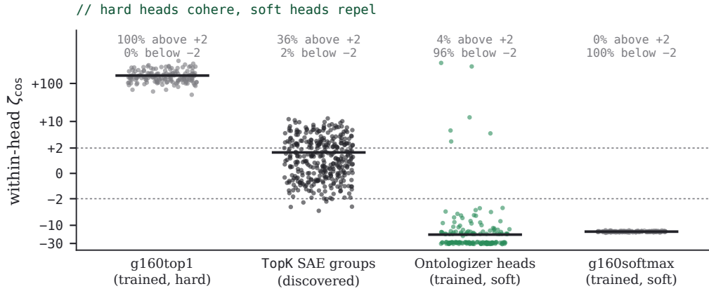
FIGURE 9 · Within-head decode-direction coherence: each head’s, or discovered group’s, \zeta_{\cos} against a size-matched null drawn from the same pool ( n_{\text{null}}=500 ), on a scale linear between the dotted lines at \pm 2 and logarithmic beyond them; bars are means. The soft heads are those of resid_nc and g160softmax , the discovered groups those of the m=11264 , k_{\text{SAE}}=32 SAE. One seed per model.
