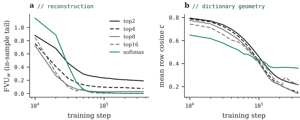
FIGURE 33 · The selection sweep’s _shm arms over training: (a) FVU_w on the (in-sample) tail, scored from each checkpoint, and (b) mean within-head row cosine \bar{c} . The soft arm’s \bar{c} flattens near 0.36 while its error keeps falling; the hard arms keep decorrelating.
