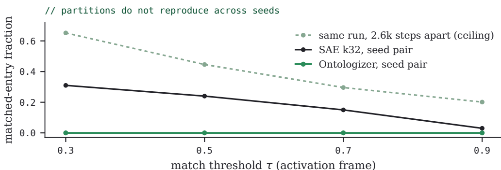
FIGURE 25 · Cross-seed matched-entry fraction on the activation frame by threshold. The same-run pair bounds what the metric can detect (0.65 at \tau=0.3 ); the k_{32} SAE pair reproduces partially; the softmax Ontologizer’s partitions reproduce not at all.
