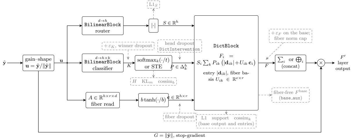
Figure 4: DictEnc with router and fibers. The gain–shape split hands the unit input \mathbf{u} to three branches: the classifier (which entry, P ), the router (how much, S , one non-negative scale per head) and the fiber read (where within the entry’s fiber, \mathbf{c} , r coordinates per head). They meet in the lookup (Equation 19); heads are summed, or concatenated under ConcatDictBlock , and the result is scaled by the measured gain G . Dashed boxes above an arrow act on it during training; dashed boxes below are statistics, which describe the fiber-free base output. That output is also returned on its own for base_aux .
