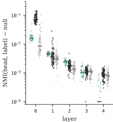
a // each head; bar = layer median
