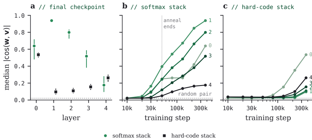
FIGURE 29 · The softmax stack’s classifier features go rank 1; the hard-code stack’s mostly do not. Median |\cos \angle(\mathbf{w}, \mathbf{v})| of each layer’s bilinear feature pairs ( bilinspec.py ), 1 for a rank-1 feature. (a) The final checkpoint by layer, with interquartile ranges: the softmax stack ( resid_nc , step 372.6k) and the hard-code stack ( ste_h76_init01 , step 369.5k). (b, c) Over training, one line per layer, numbered at its end; the softmax stack’s temperature anneal ends at 50k, and the hard-code stack’s temperature is constant. Dashed: the median for a random pair in the 1024-dimensional semantic block, 0.021. One seed per run.
