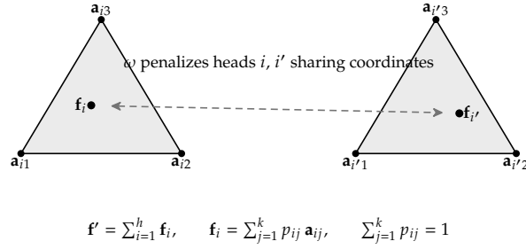
FIGURE 4 · DictBlock head geometry for h=2 ; k=3 . The output space of a head i is a simplex with its atoms \mathbf{a}_{ij} , the rows of |D_i| , as vertices. The assignment P is a soft choice among mutually contrastive categories rather than a set of independently firing features, and because p_{ij} \in [0, 1] the output lies within the convex hull of the head's atoms. Because |D| \geq 0 and P \geq 0 , F \geq 0 , so \cos \angle(\mathbf{f}_i, \mathbf{f}_{i'}) \in [0, 1] , and driving the support overlap \omega to zero asks the heads to partition the coordinates of \mathbb{R}^e between them (§5.1.3).
