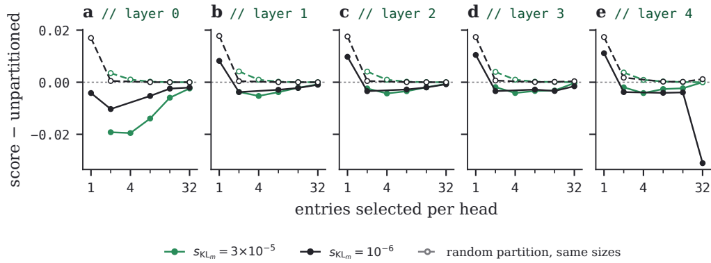
FIGURE 34 · Partitions barely beat a plain smoother. The selection sweep’s held-out noise2self score per layer, against the number of entries each head selects (1 is argmax, 32 is softmax), less the same run’s score with every row in one cell (below 0 the partition helps), for the two mean-entropy bonus settings. Filled: the heads’ partitions, mean over heads; hollow, dashed: the same assignments with the rows permuted, a random partition with matched cell sizes. Heat kernel of bandwidth 0.2 on the layer’s input, batches of 2,048 rows. One seed per arm, in-sample tail.
