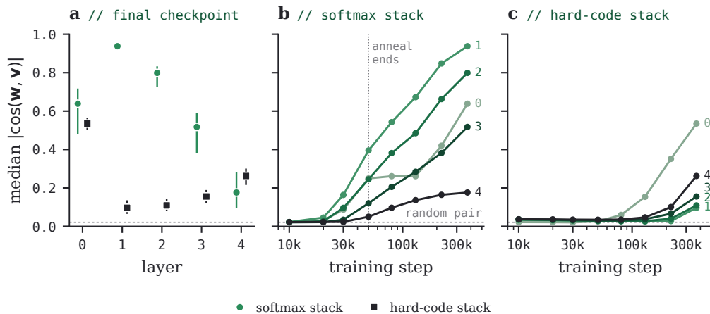
FIGURE 35 · The softmax stack’s classifier features go rank 1; the hard-code stack’s mostly do not. Median |\cos \angle(\mathbf{w}, \mathbf{v})| of each layer’s bilinear feature pairs (bilinspec.py), 1 for a rank-1 feature. (a) The final checkpoint by layer, with interquartile ranges: the softmax stack (resid_nc, step 372.6k) and the hard-code stack (ste_h76_init01, step 369.5k). (b, c) Over training, one line per layer, numbered at its end; the softmax stack’s temperature anneal ends at 50k, and the hard-code stack’s temperature is constant. Dashed: the median for a random pair in the 1024-dimensional semantic block, 0.021. One seed per run.
