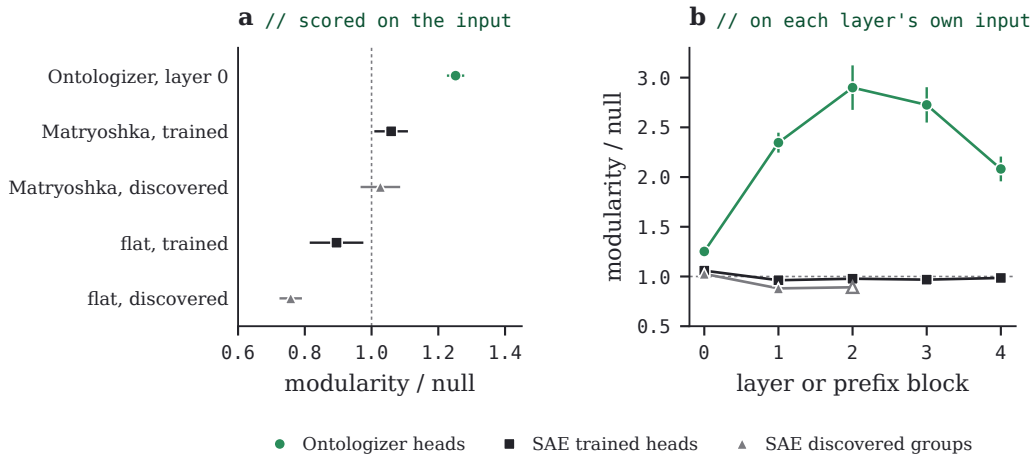
FIGURE 17 · Ontologizer heads are communities of the residual they classify; SAE heads and groups are not. Soft modularity over its size-matched null ( headstruct.py -modularity, Eq. (35)); bars are \pm 2 null standard deviations. (a) Every model scored on the input itself: the softmax Ontologizer’s layer 0, block 0 of the two Matryoshka SAEs (scored on \mathbf{x} - \mathbf{b}_{\text{dec}} , the SAE encoder’s input), and the two flat SAEs. (b) By depth, each layer or prefix block on the graph of its own input. Hollow: a block whose groups cover under 10% of samples. The discovered groups’ blocks 3 and 4 are not drawn: block 3’s null is within two of its standard deviations of 0 (3% coverage), and block 4 holds one group, which its null reproduces exactly. One checkpoint per model.
