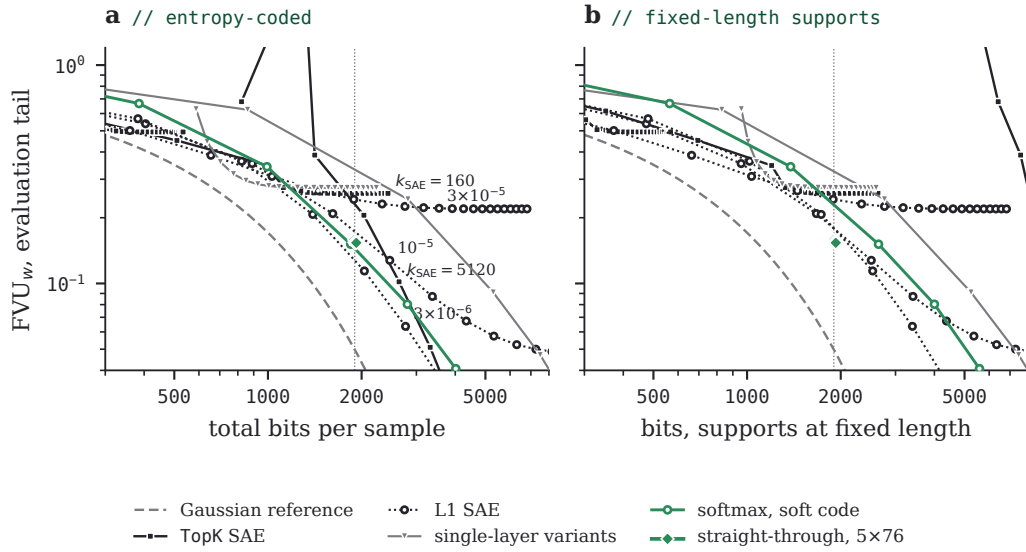
FIGURE 29 · Operational rate on the evaluation tail: everything each code sends quantized (Eq. (26)) at a swept step, (a) each slot’s symbols entropy-coded and (b) each support charged its fixed-length cost, the values still entropy-coded. L1 SAEs are labeled by s_{L1} ; the unlabeled TopK curve is k_{SAE}=32 , and the single-layer variants are g160top1 (level) and g160softmax (falling). The straight-through stack’s curve spans 1895–1923 bits. The dotted line is 1900 bits and the dashed curve the Gaussian reference (Eq. (25)). The softmax model saw the tail in training; scored on rows no model saw, no curve’s readout at 1900 bits moves by more than 0.0004 (Appendix B.1). One seed per curve.
