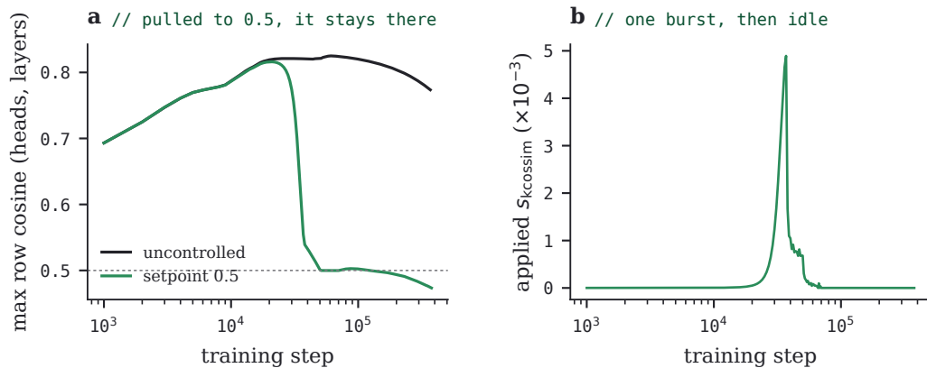
FIGURE 32 · The row-collinearity setpoint on the shipped stack, from the training log. (a) The max within-head row cosine over heads and layers, the statistic the controller watches, against the uncontrolled twin; the dotted line is the 0.5 setpoint. (b) The applied multiplier s_{kcossim} , averaged over 1000-step windows.
