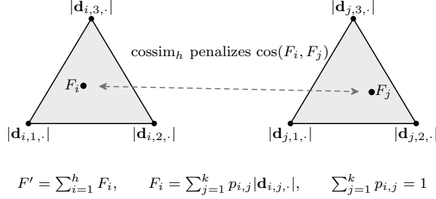
Figure 3: DictBlock head geometry for h = 2 ; k = 3 . The output space of a head i forms a simplex with the rows of the matrix D_{i,\cdot,\cdot} as the vertices. The row vectors \mathbf{d}_{i,j,\cdot} form the spanning set of the feature space. Any F_i must be a linear combination of the rows of D_{i,\cdot,\cdot} . As F becomes sparser, these vectors become more approximately orthogonal, allowing them to be treated as a basis. The label code P corresponds to soft assignments to mutually contrastive categories rather than independently firing features. Because elements of P , p_{ij} \in [0, 1] , outputs must be within the convex hull of D_{i,\cdot,\cdot} . Because |D| \geq 0 and P \geq 0 , F \geq 0 ; therefore \cos(F_i, F_j) \in [0, 1] , and driving \text{cossim}_h(F) to zero asks the heads to partition the coordinates of \mathbb{R}^e between them (Section 3.1.4).
