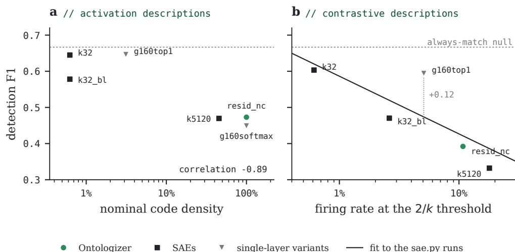
FIGURE 11 · Mean detection F1 per run of Table 6 against code density. (a) Activation descriptions against nominal density, the share of a code’s coefficients that are nonzero. (b) Contrastive descriptions against the firing rate at the 2/k threshold, with a line fitted in log rate to the four sae.py runs that fire; gl60softmax never crosses the threshold and is not drawn, and the Ontologizer ( resid_nc ) is held out of the fit. Detection sets are half positives, so a description that matches every item scores the always-match null, 2/3 (dotted). One seed per run.
