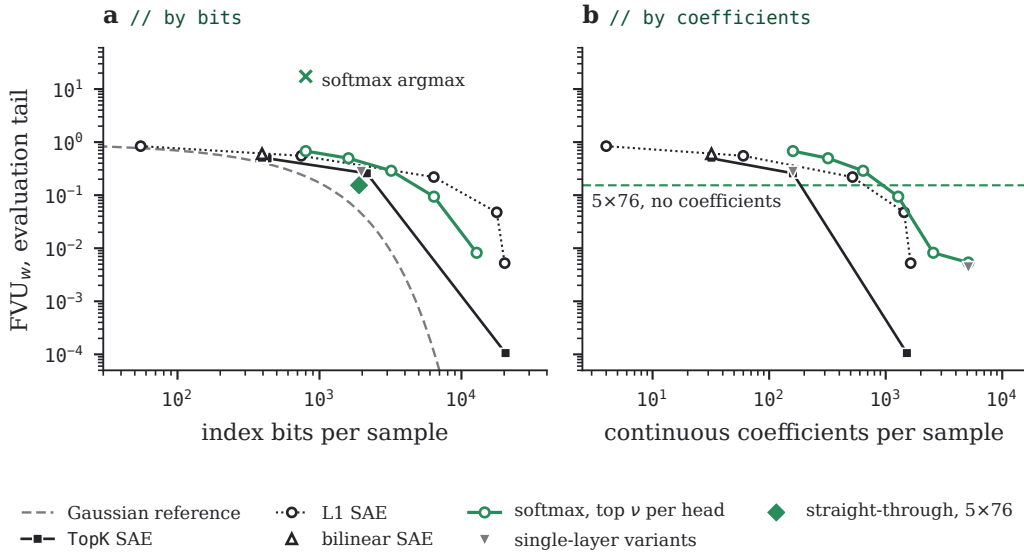
FIGURE 8 · Reconstruction against code size on the shared evaluation tail, by index bits (a) and by continuous coefficients (b): the points of Table 1, the L1 SAEs at all five weights, and the straight-through stack (ste_h76_init01, Section 5). A code appears only where its size is nonzero, so the soft codes are in (b) alone, the softmax argmax is in (a) alone, and the straight-through stack is a level in (b). The dashed curve is the Gaussian reference (Eq. (25)). The softmax model (resid_nc) saw the tail in training and the others hold it out. One seed per point, except the k_{\text{SAE}}=32 SAE’s seed-43 replica.
