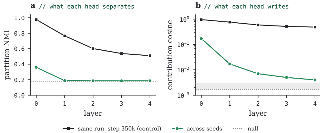
FIGURE 12 · Table 8 by layer: what each head separates (a, partition NMI) and what it writes (b, centered contribution cosine, log scale), across the two seeds and against the first run’s own checkpoint at step 350,000. Dotted lines are the nulls; the band in (b) runs from the null’s mean to its maximum. One seed pair.
