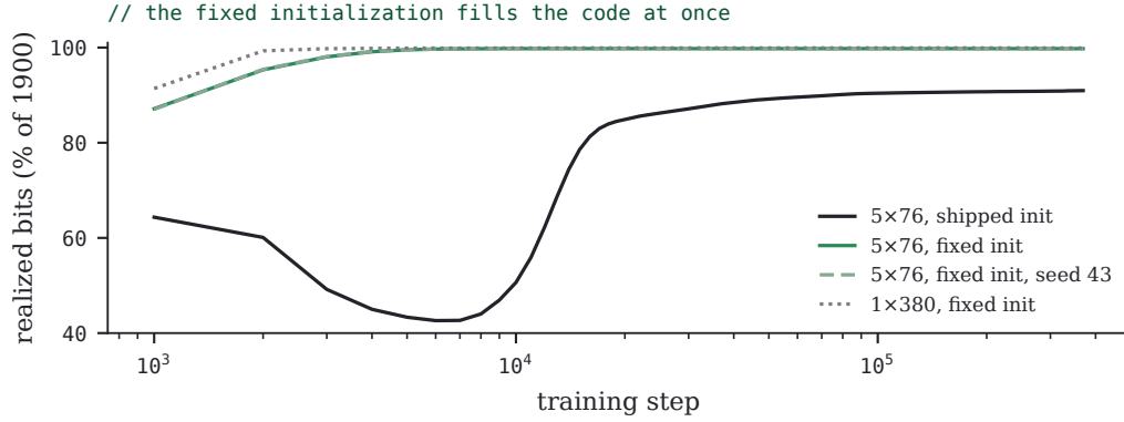
FIGURE 24 · Realized code bits over training, as a share of the nominal 1900, from the logged KL_m less its one-batch sampling floor. The shipped initialization’s head usage collapses to under half before recovering to 90% (the curve’s 91% over-corrects heads with dead entries); at the fixed initialization every head in the stack and the flat arm reaches near-uniform usage within 5k steps. An upper bound on the information carried, not a measure of it (Eq. (34)).
