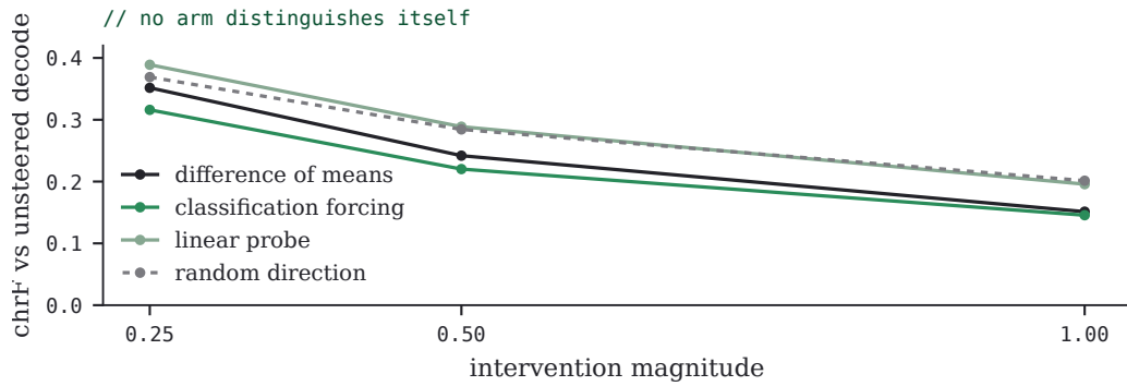
FIGURE 22 · chrF between steered and unsteered decodes by intervention magnitude. All four arms, the random direction included, damage the decode at nearly the same rate; no arm buys naturalness at matched magnitude.
