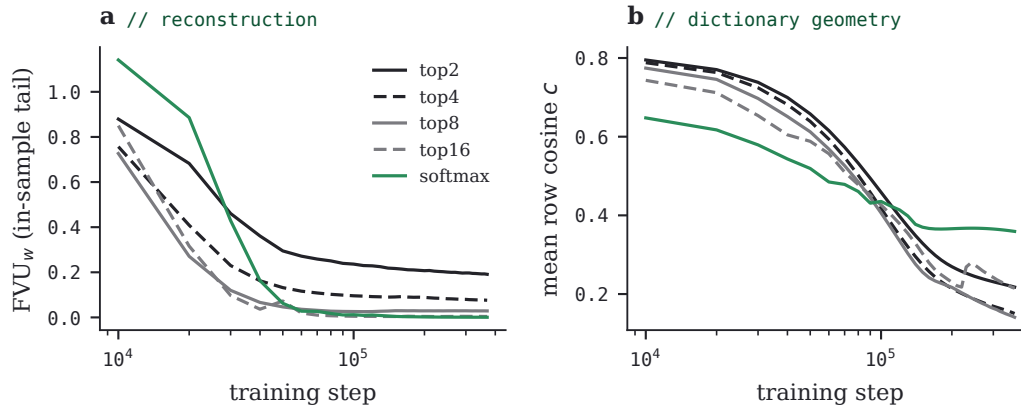
FIGURE 27 · The selection sweep’s _shm arms over training: (a) FVU_w on the (in-sample) tail, scored from each checkpoint, and (b) mean within-head row cosine \bar{\kappa} . The soft arm’s \bar{\kappa} flattens near 0.36 while its error keeps falling; the hard arms keep decorrelating.
