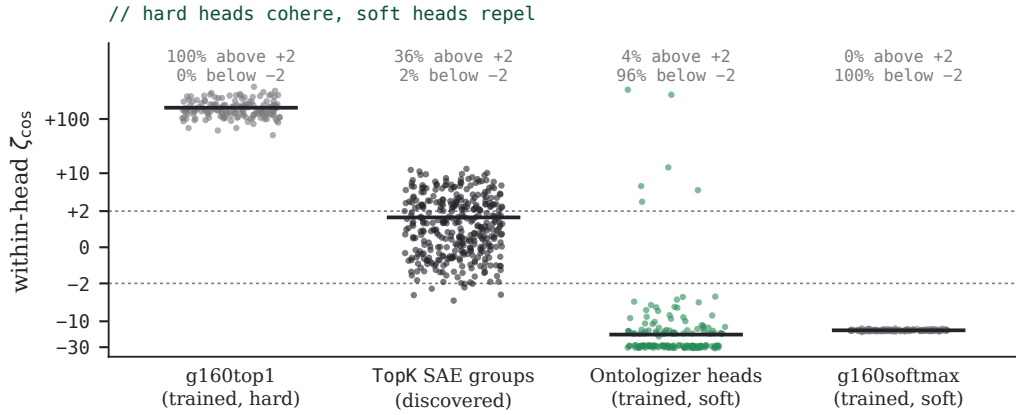
FIGURE 9 · Each head’s, or discovered group’s, \zeta_{\cos} against its size-matched null (Table 3), on a scale linear between the dotted lines at \pm 2 and logarithmic beyond them; bars are means. The soft heads are those of resid_nc and g160softmax , the discovered groups those of the m=11264 , k_{\text{SAE}}=32 SAE. One seed per model.
