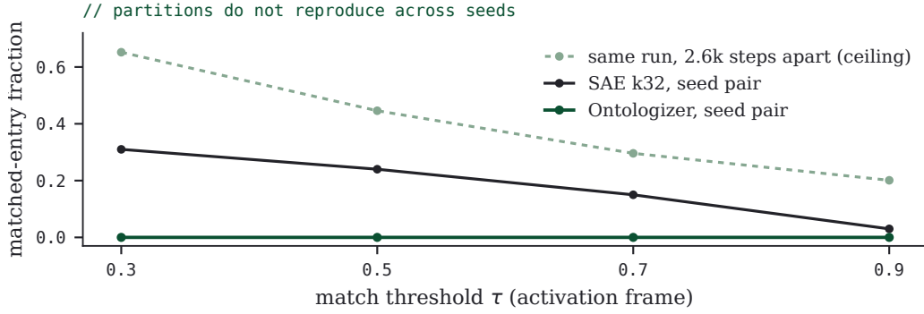
FIGURE 12 · Cross-seed matched-entry fraction on the activation frame by threshold. The same-run pair bounds what the metric can detect (0.65 at \tau=0.3 ); the k32 SAE pair reproduces partially; the softmax Ontologizer’s partitions reproduce not at all.
