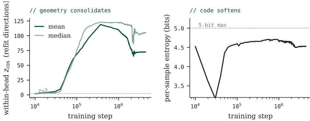
FIGURE 10 · The 448-checkpoint training history of resid_nc_hm . Left: within-head coherence of refit end-to-end directions, z-scored against size-matched nulls; rise, peak near step 370k, partial relaxation. Right: mean per-sample classification entropy returns toward the 5-bit maximum after the annealing transient.
