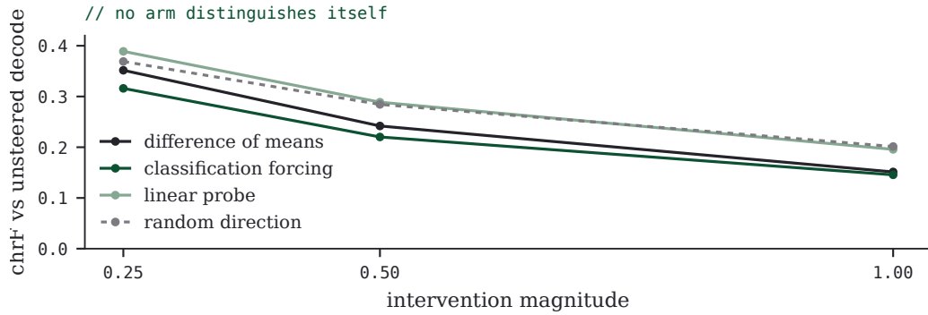
FIGURE 13 · chrF between steered and unsteered decodes by intervention magnitude. All four arms, the random direction included, damage the decode at nearly the same rate; no arm buys naturalness at matched magnitude.
