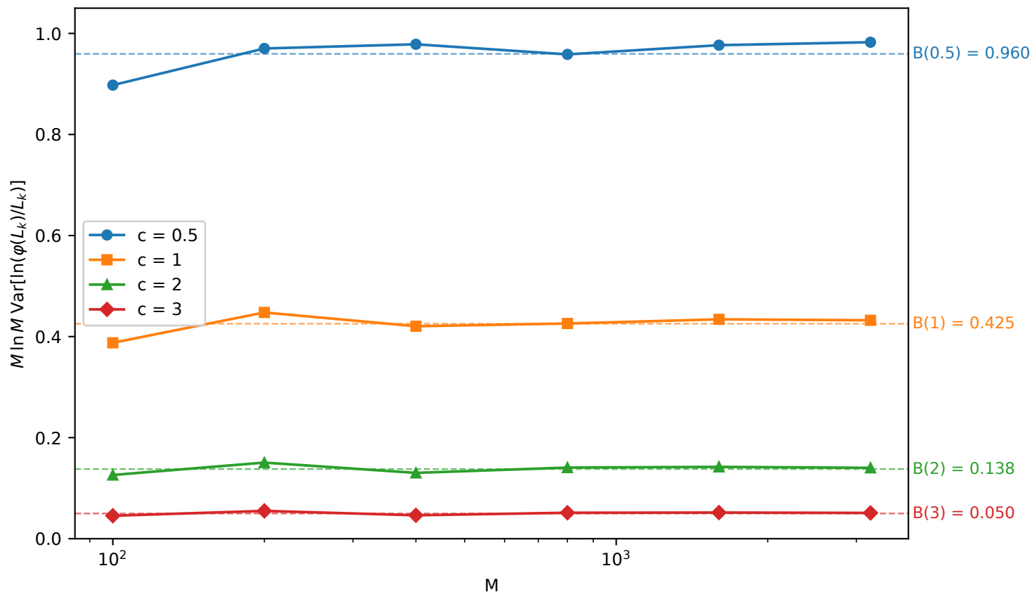
Convergence of the rescaled variance to B(c) , at k = \lfloor cM \rfloor
