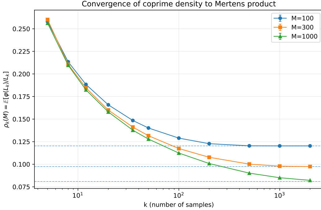
Figure 1: Monte Carlo estimates of \rho_k(M) for M \in \{100, 300, 1000\} , based on N = 2000 independent replicates per point. Error bars show \pm 1 standard error of the sample mean. Dashed lines indicate the exact Mertens product P_M .
